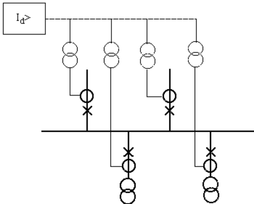
Figure 1. A one zone differential relay for a single busbar.
