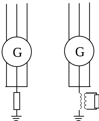
Figure 5. Two equivalent methods for high resistance earthing.
