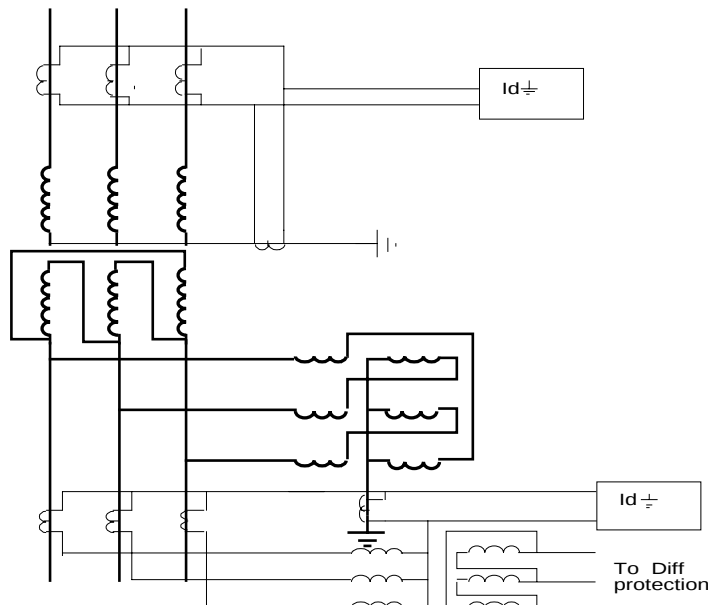
Figure 12. A Restricted earth fault relay in a reactance earthed system with a Z-0 transformer.
