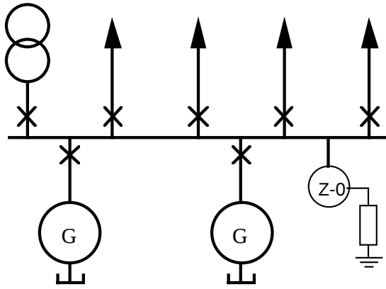
Figure 13. Earthing, with a Z/O-connected transformer on the busbar.
