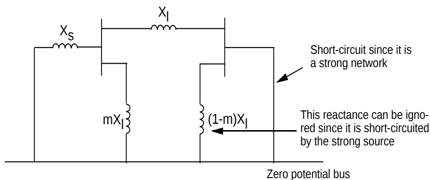
Figure 7. Thevenins theorem applied on the faulty network.
