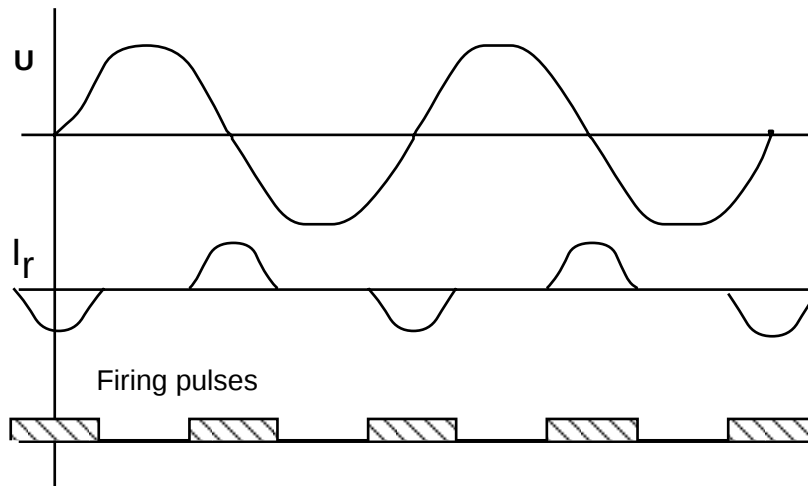
Figure 3. Voltage and current wave form and thyristor firing control.
