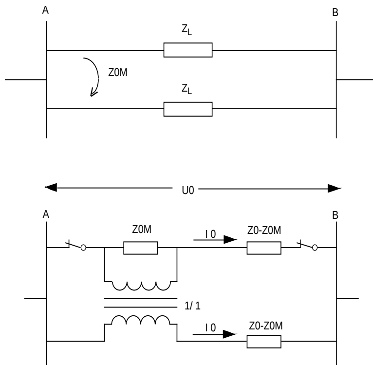
Figure 15. Influence of mutual impedance, at parallel lines, at the same tower.
