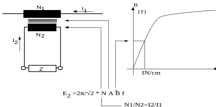
Figure 2. The factors influencing the current transformers output and magnetizing current.
