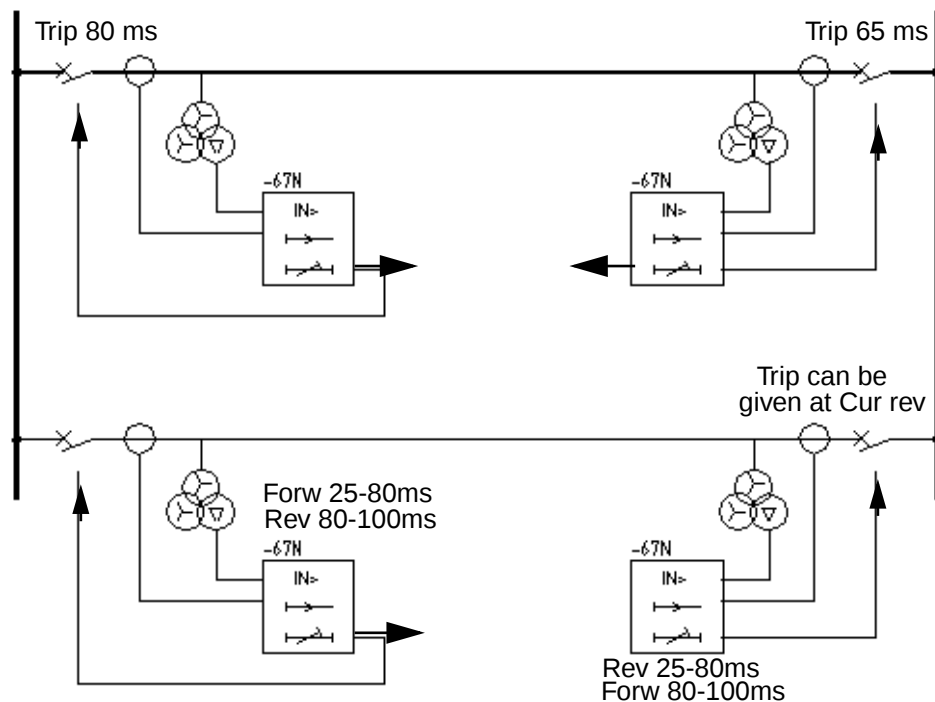
Figure 9. The current reversal problem at parallel lines.
