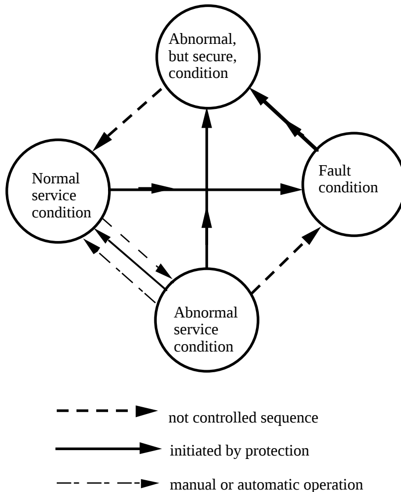
Figure 1. The power system's operation conditions.
