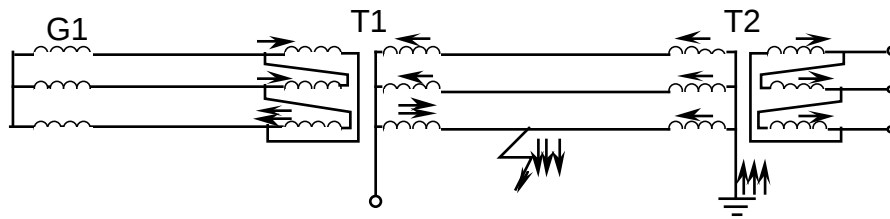
Figure 9. Current distribution in a transmission network.
