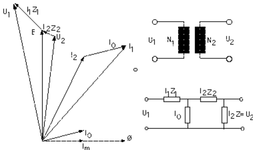
Figure 1. The principle of an Instrument transformer.
