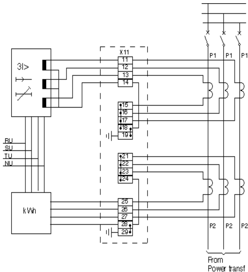
Figure 4. A terminal arrangement which allows simple reconnection of a current transformer direction and a simple testing of each core.
