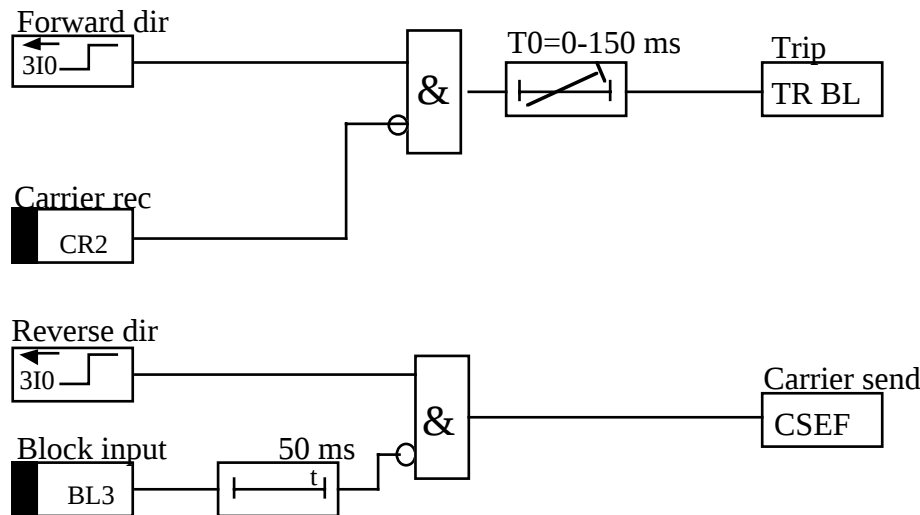
Figure 8. A blocking scheme with directional earth fault relays.
