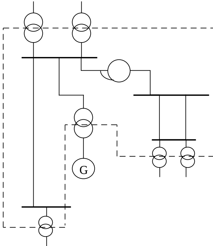
Figure 1. The earthing of a system is effective for all galvanic connected parts.
