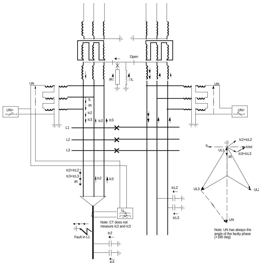
Figure 16. A Directional earth fault relay on a resonance earthed system.
