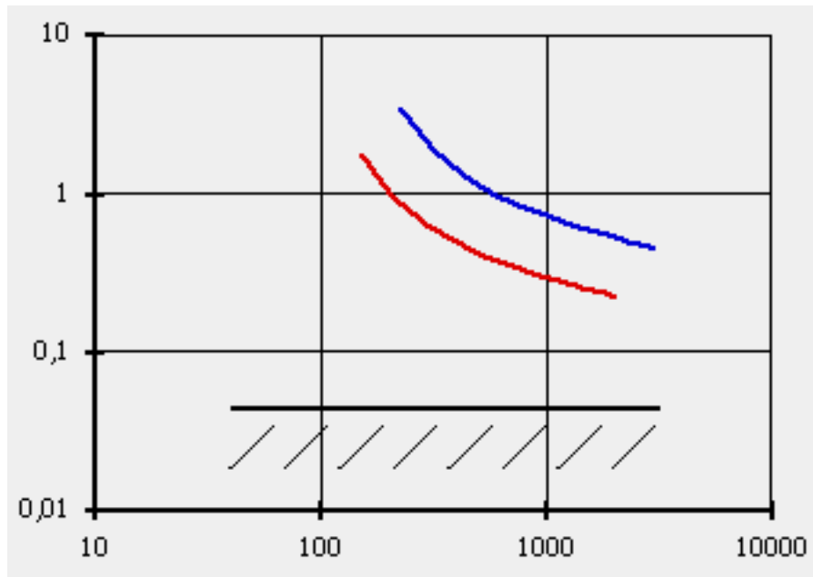
Figure 19. A Differential relay can be indicated in the selectivity plan with the operating time and a current range starting from maximum sensitivity.
