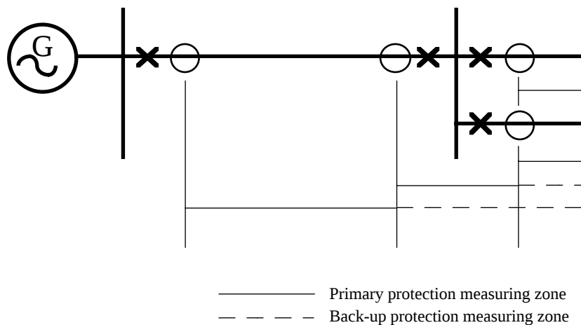
Figure 4. Primary and back-up protection zones
