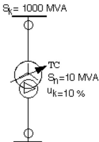
Figure 14. For a transformer an instantaneous stage can be used as the impedance of the transformer will limit the fault current at a low voltage fault.
