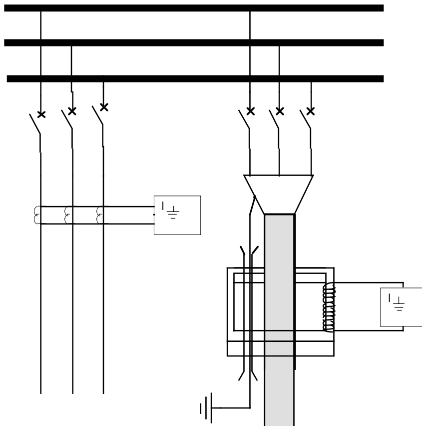
Figure 20. Measurement of earth fault current can be made with a residual sum measurement of a cable CT surrounding all three phases.
