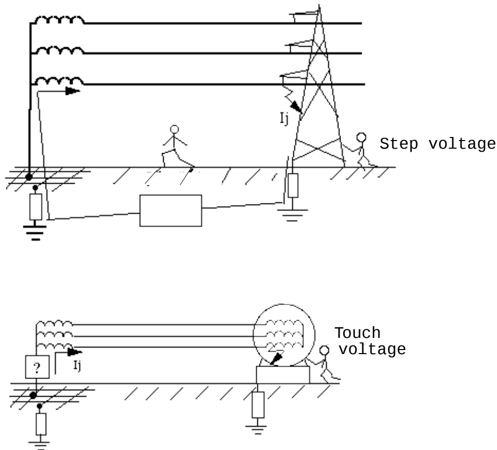
Figure 15. How the step and touch voltages, arises in a direct earthed network.
