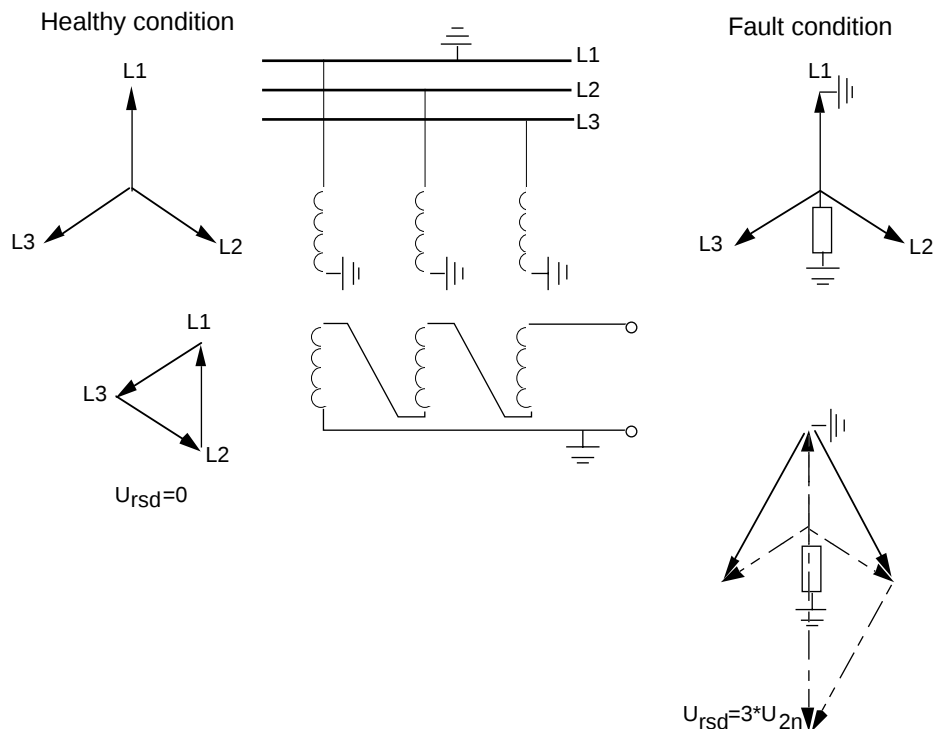
Figure 6. The principle for an open delta winding. Occurring voltages at an earth fault in a unearthed or high resistive/resonance earthed system.
