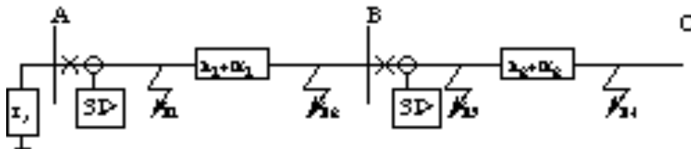
Figure 10. A Fuse and time selective overcurrent protection.
