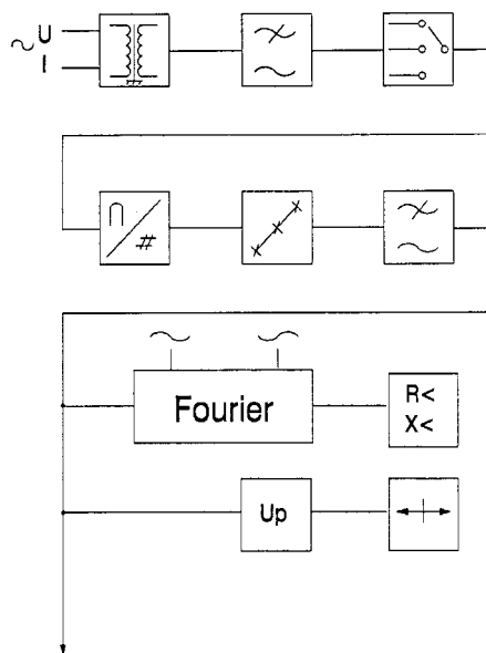
Figure 9. The design of a Numerical distance protection relay.
