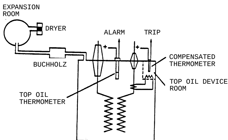
Figure 4. Location of buchholz, top oil thermometer and winding temperature indication
