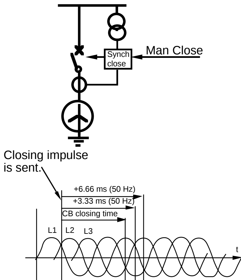
Figure 2. Synchronized closing of Shunt Reactor Circuit Breakers.
