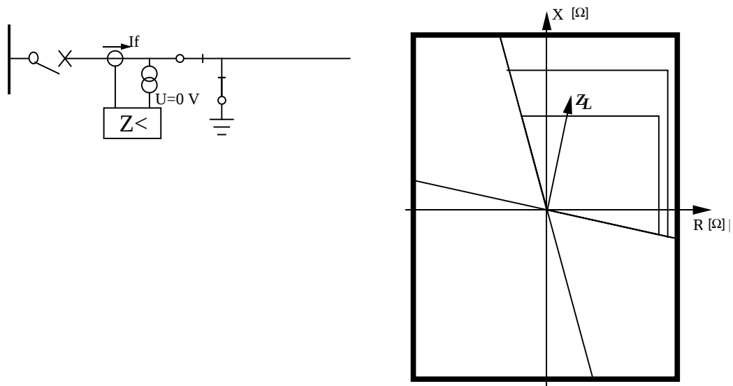
Figure 16. Switch Onto Fault function ensures fast tripping when energizing a line onto a forgotten earthing.
