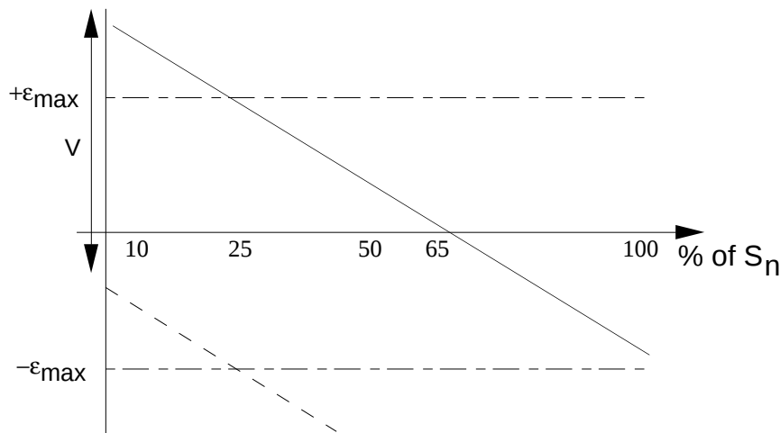
Figure 3. The measuring error as a factor of secondary burden at a constant primary voltage.
