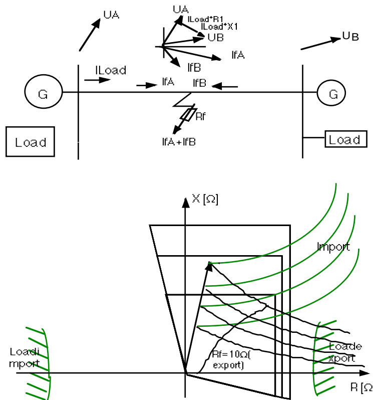
Figure 14. Measuring error at a high resistive earth fault in a line with double side infeed.
