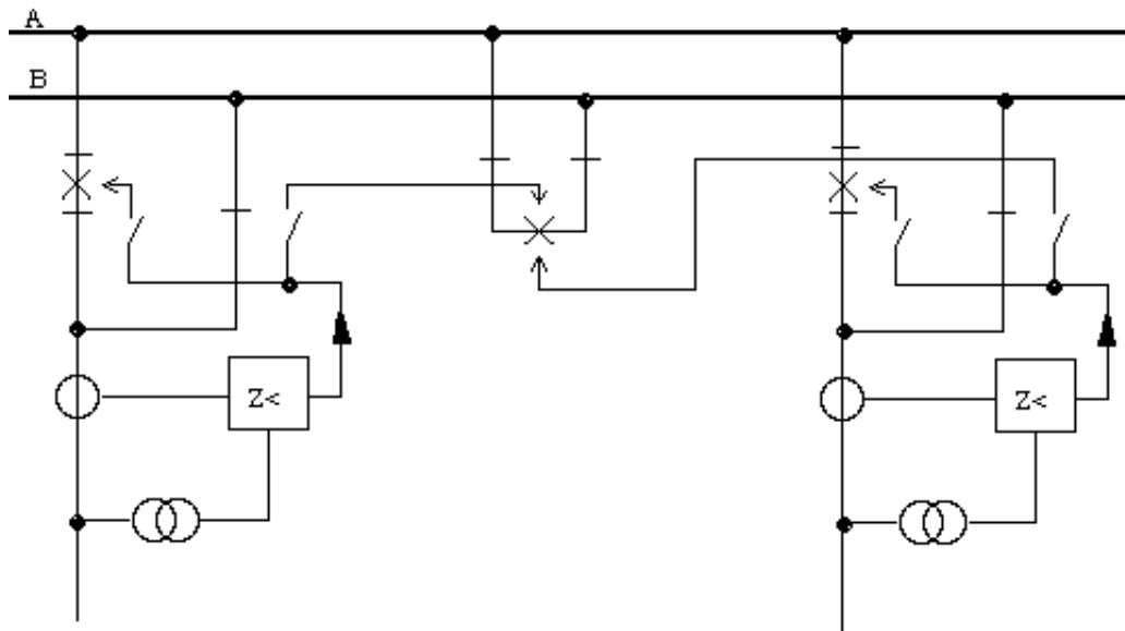
Figure 2. The location of current transformer at a AC-Busbar arrangement.
