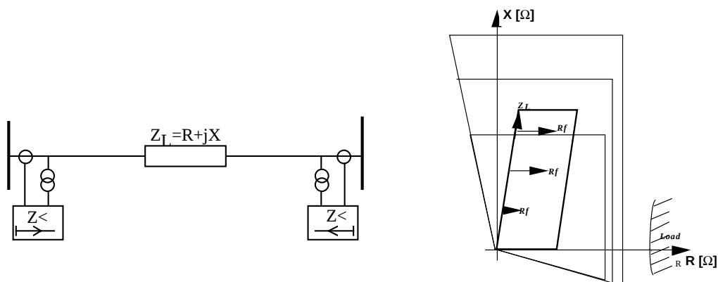
Figure 7. The principle of a Distance protection relay.
