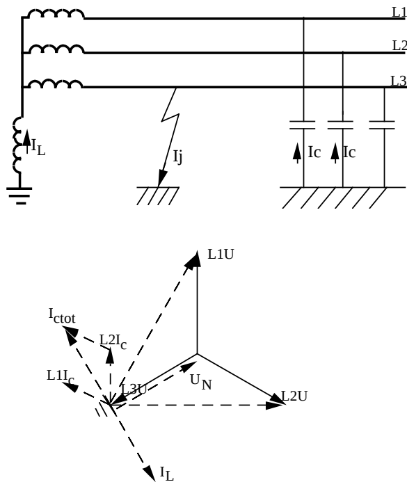
Figure 2. Reduction of earth fault current with a neutral-point impedance. Resulting earth fault current I_j is very small if I_L = I_{CTot}
