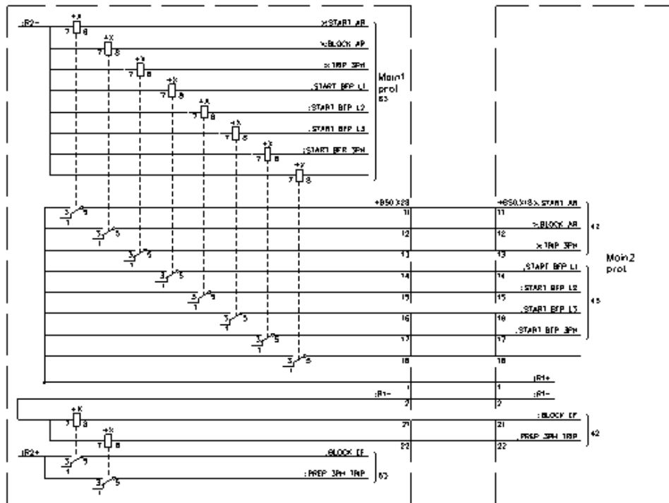
Figure 5. Sub 1 -Sub 2 interface for a HV overhead line
