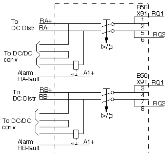
Figure 8. Supervision of the DC supply to a protection panel, detecting faulty supply fuse, open circuit and DC/DC converter failures.
