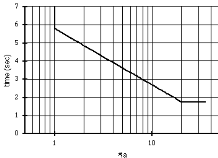
Figure 6. The logarithmic inverse characteristic. A fault current of the biggest infeed less than 0,8 times the current of the faulty object, gives a selective tripping.
