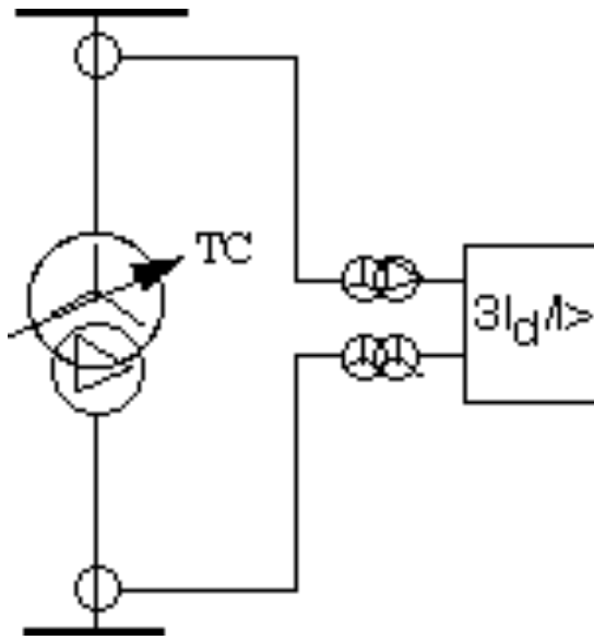
Figure 7. The differential relay for a transformer needs to have phase angle shift compensation and must have a percentage restraint to operate correctly for through faults as the tap changer percentage error will be increased at through faults. Stabilization is achieved with a summation (I_1 + I_2)/2
