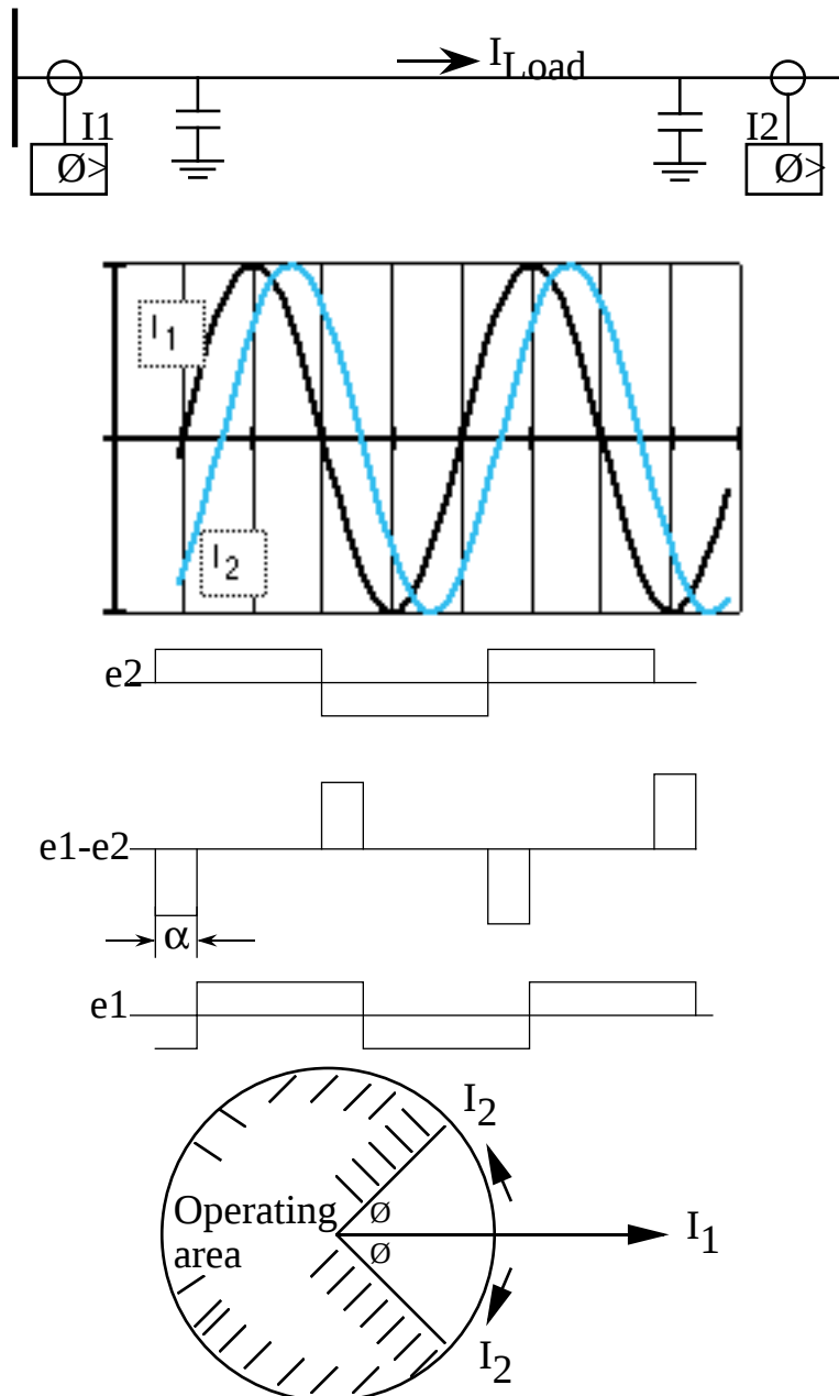
Figure 6. Measuring principle of a phase comparison relay. The angle difference, between the currents at the two line ends, is compared.
