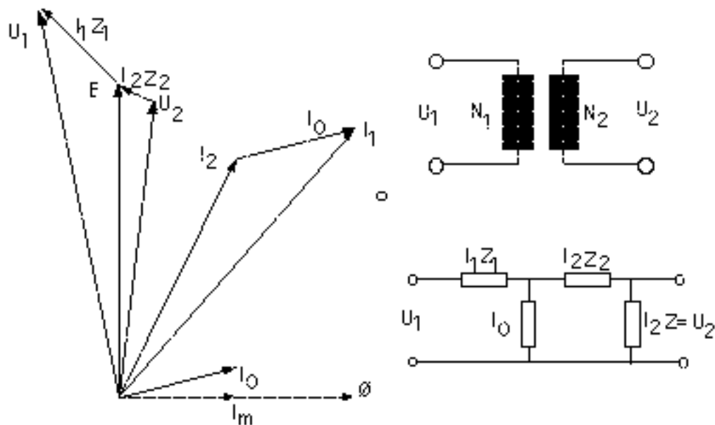
Figure 1. The principle of an instrument transformer.
