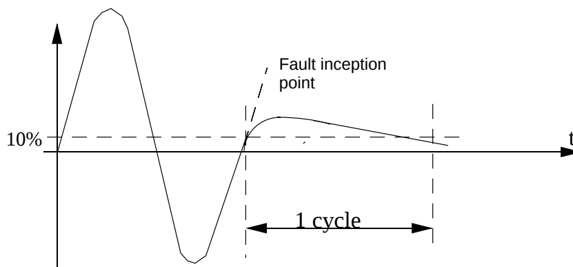
Figure 7. The transient voltage at a solid short circuit on the terminals of a Capacitive voltage transformer.
