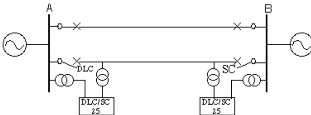
Figure 30. Dead line check (DLC) and synchronism check (SC) at auto-reclosing. 25 = DLC/SC device
