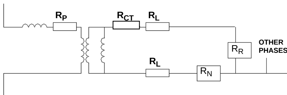
Figure 1. The current transformer principle circuit with magnetizing reactance and secondary resistance.
