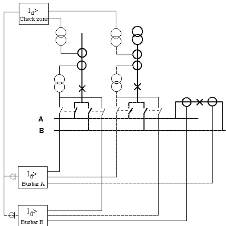
Figure 4. 2-zone busbar differential protection, for double busbar switchgear (including check zone), releasing the main zones for busbar A and B.
