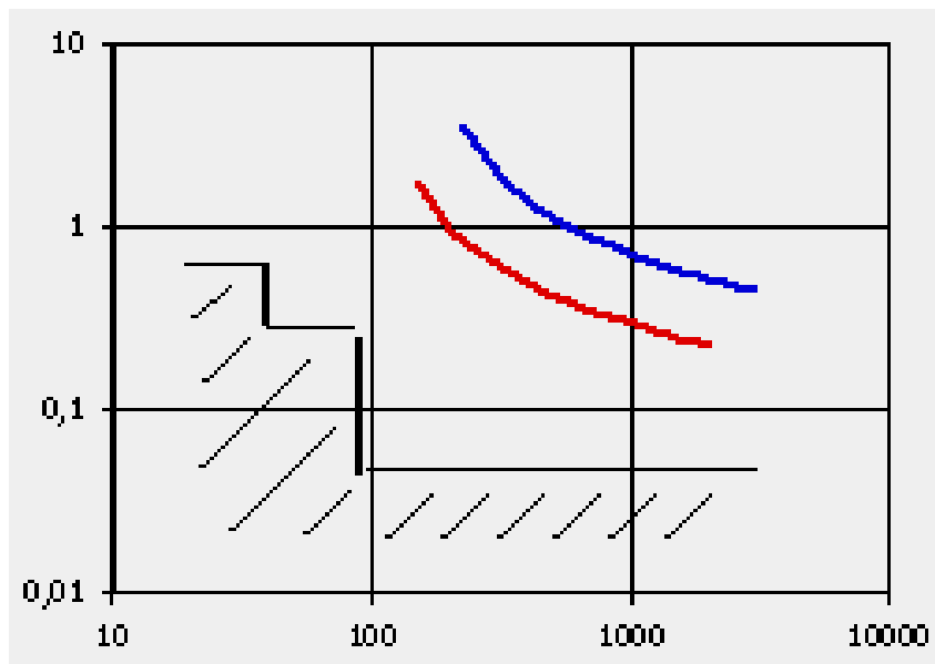
Figure 20. A Distance protection with three stages can be indicated with the time stages and impedance stages recalculated to MVA or current at nominal voltage and possible some other voltage level as a range for each stage.
