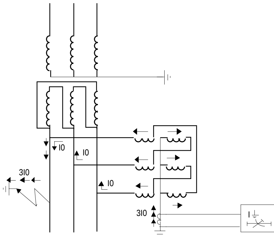
Figure 11. The principle of a Zig-zag transformer providing earth fault current in a reactance earthed system.
