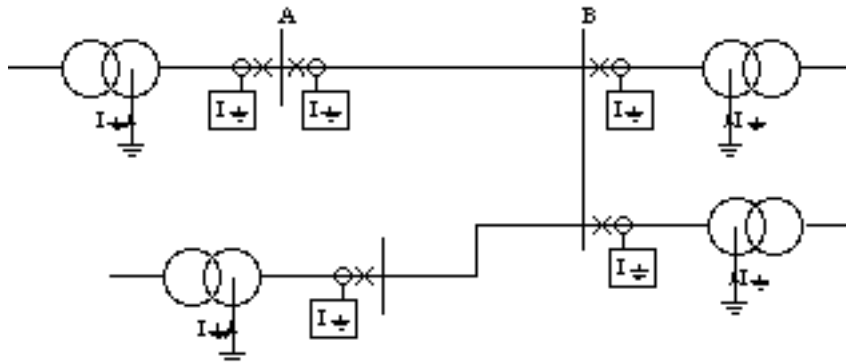
Figure 16. The earth fault protection relays in a solidly earthed system.
