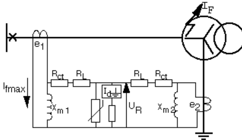
Figure 8. The connection and principle for a Restricted Earth Fault protection (REF)
