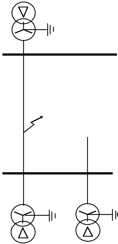
Figure 1. An earth fault in a direct, effectively earthed system.
