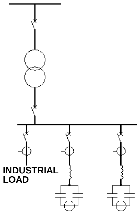
Figure 1. Capacitor banks with series reactors.
