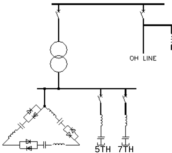
Figure 4. Thyristor controlled reactors (TCR).
