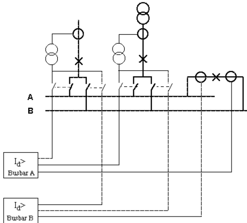
Figure 3. 2-zone busbar differential protection, for double busbar switchgear.
