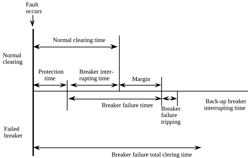
Figure 8. Time scheme for breaker failure relays
