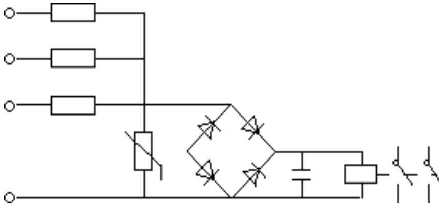
Figure 5. Supervision of a voltage transformer circuit (for alarm purpose only).
