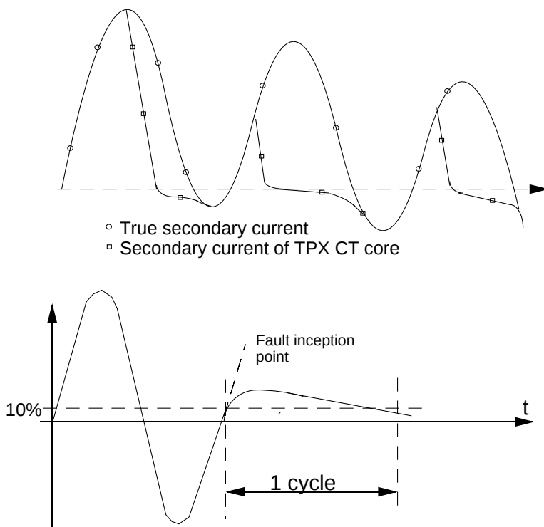
Figure 11. Output signals from a DC saturated current transformer and from a CVT at a close-up fault.
