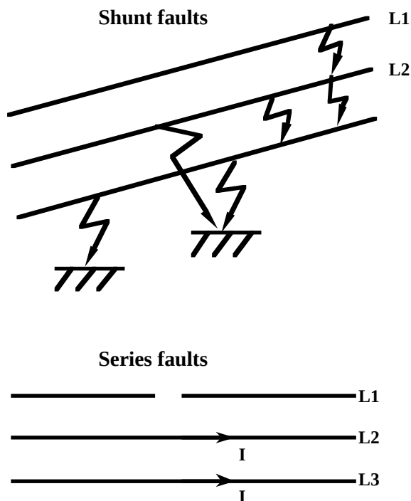
Figure 2. Different fault types in a power system.
