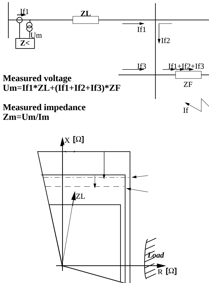
Figure 13. The Distance protection underreach at a remote fault.
