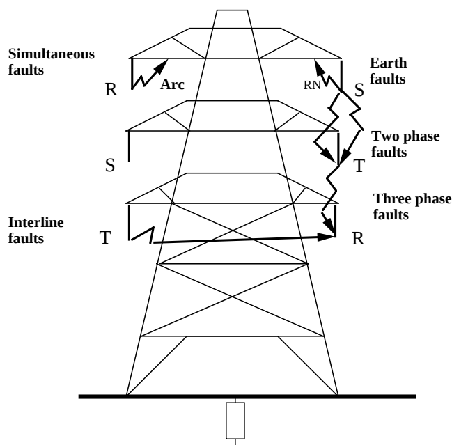
Figure 1. Faults occurring on a transmission line tower are of different types.
