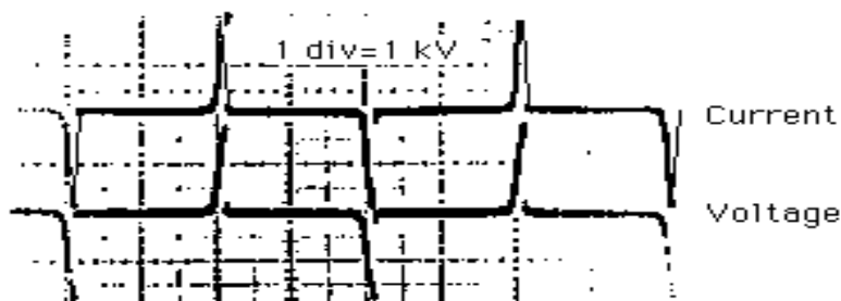
Figure 4. The high impedance principle.
