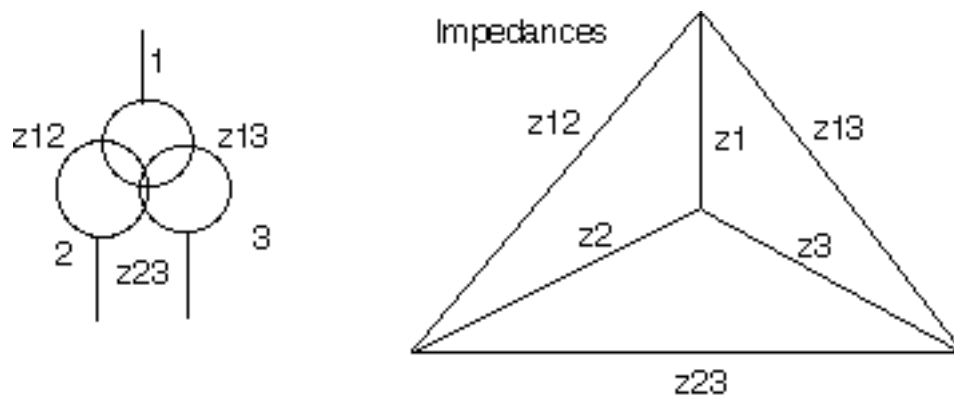
Figure 1. The Star delta impedance transformation is necessary to calculate fault currents when three winding transformers are involved.
