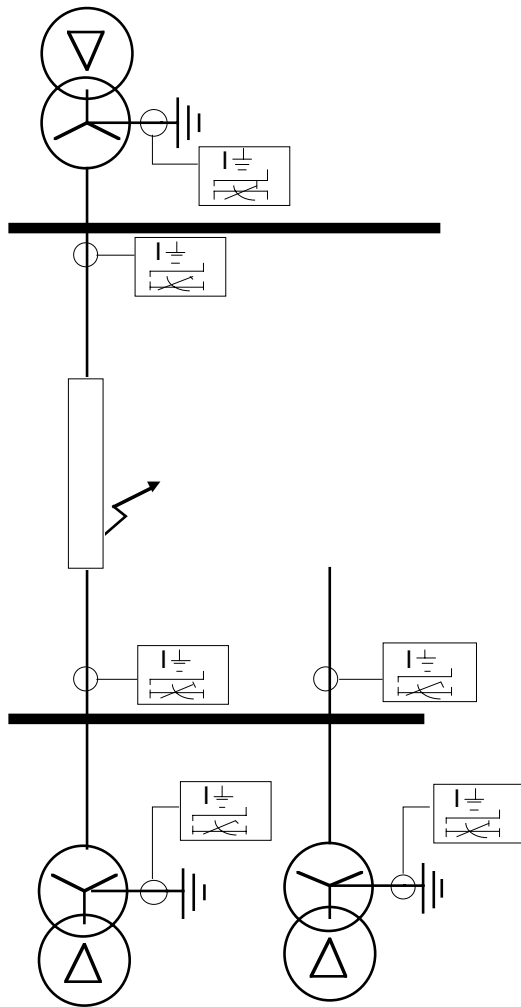
Figure 5. Earth fault protection in a solidly earthed system.
