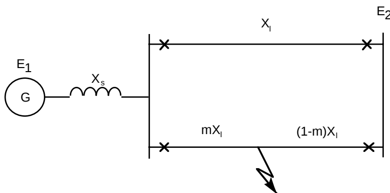
Figure 6. Line fault on one circuit of a double Overhead line.
