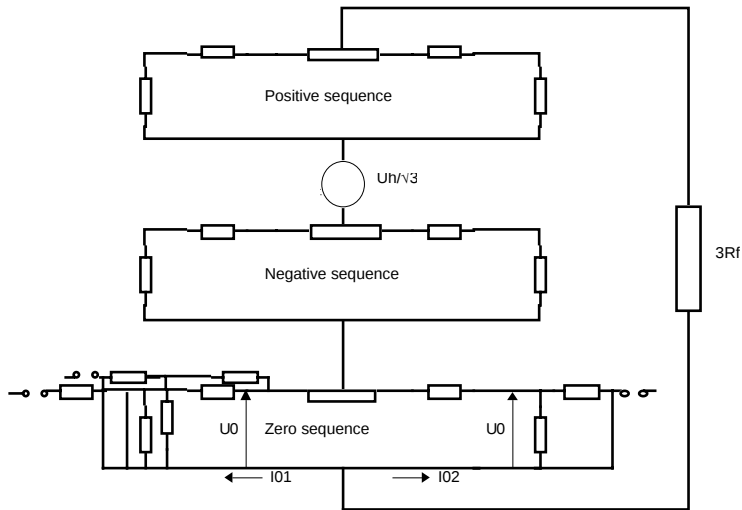
Figure 2. The symmetrical components are used to calculate the " I_0 " current for the fault in figure 1, " 3I_0 " is the total fault current.
