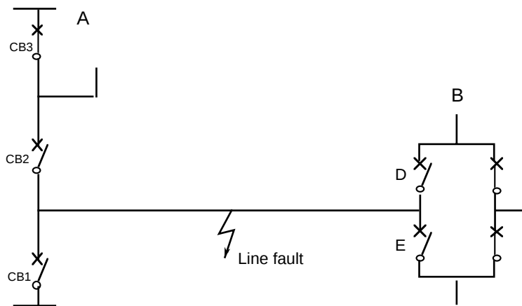
Figure 27. Some Auto reclosing sequences in multi breaker systems.
