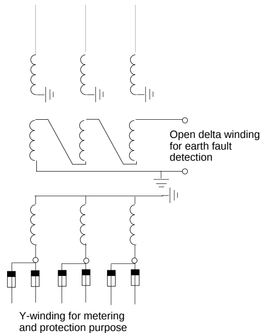
Figure 4. A Voltage transformer with two secondary windings, one Y-connected and one Open delta connected.
