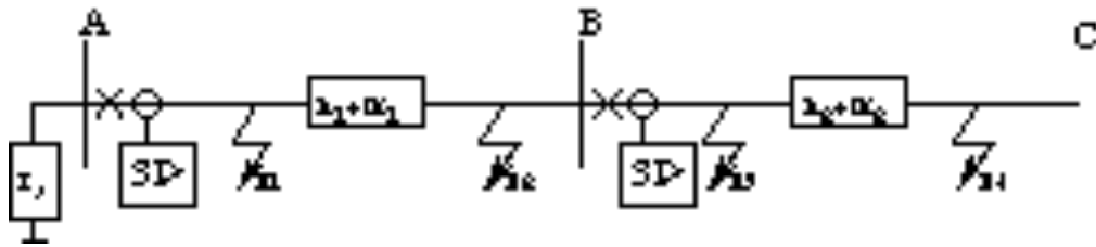
Figure 9. Current selective relays at A and B.
