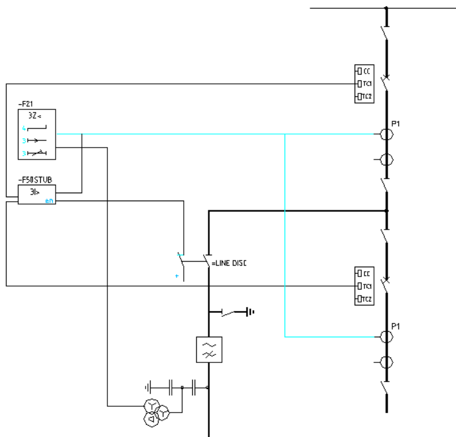
Figure 18. Stub protection function protects the line exit when the line disconnecter is open.
