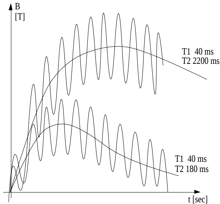
Figure 3. AC and DC flux dependent of time, at faults with full DC component and with different primary and secondary time constants.
