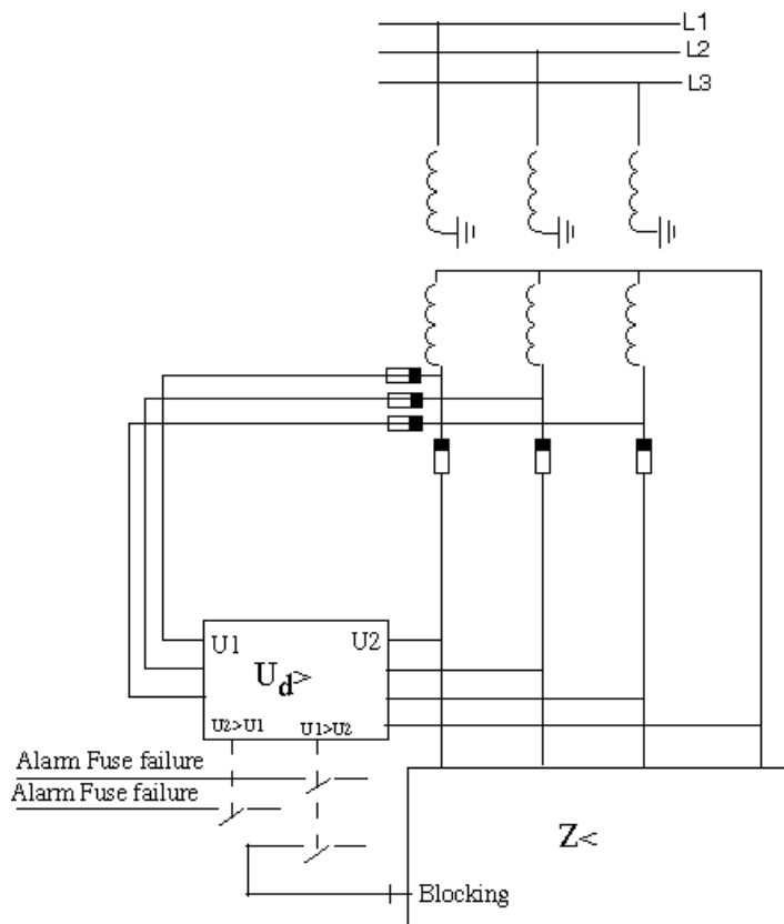
Figure 6. Supervision of a Voltage transformer secondary circuit (for blocking of protection).
