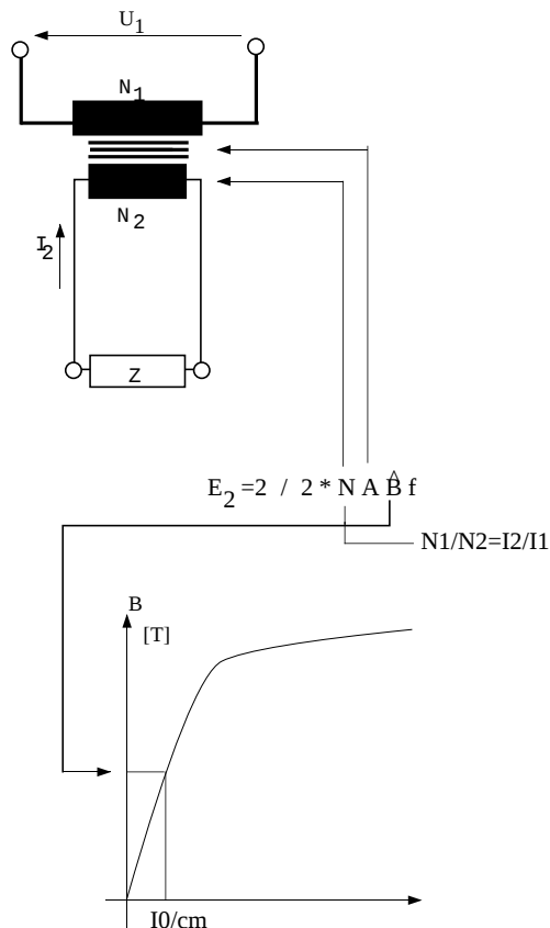
Figure 2. The factors influencing the voltage transformer output and magnetizing current.
