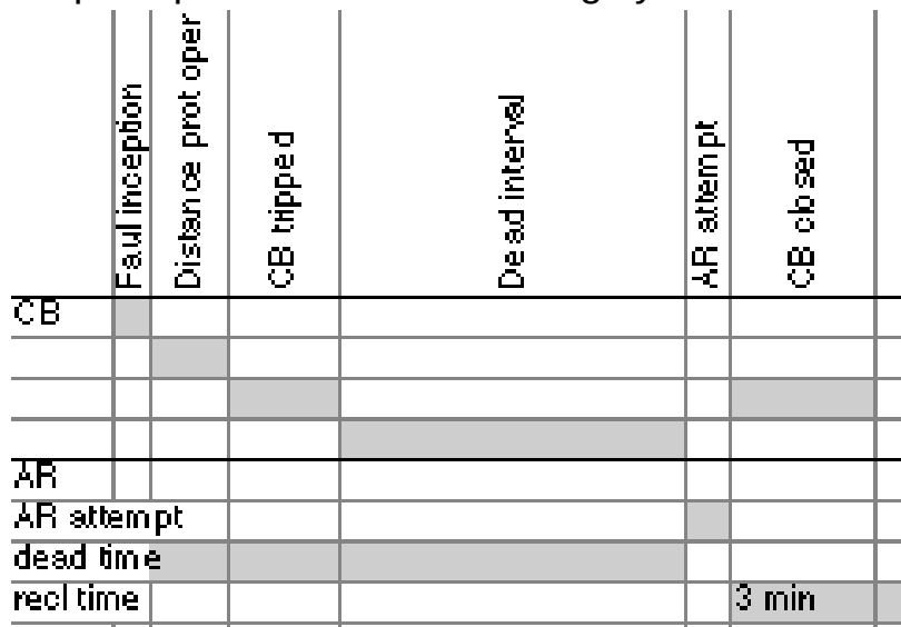
Figure 23. The operating principle of an Auto reclosing device.
