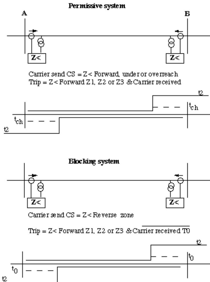
Figure 2. The principle for Distance protection relays communication.
