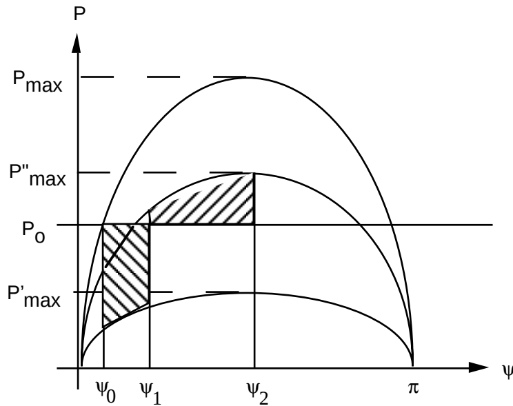
Figure 8. The equal area method shows the stability limit.
