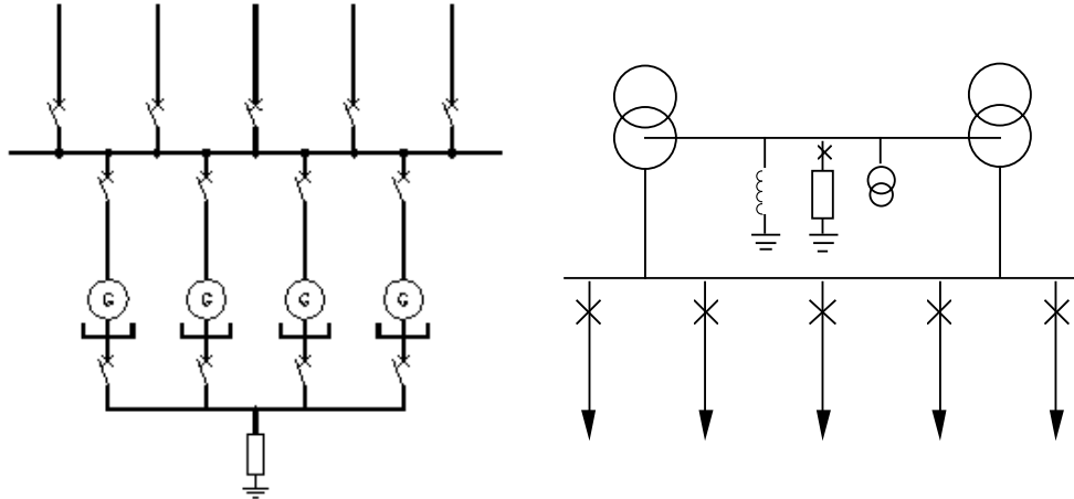
Figure 11. Resistance earthing, of the generator neutral-point, with a neutral busbar and individual neutral-point breakers.
