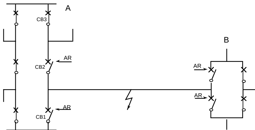
Figure 24. Auto reclosing of transmission line CB:s.
