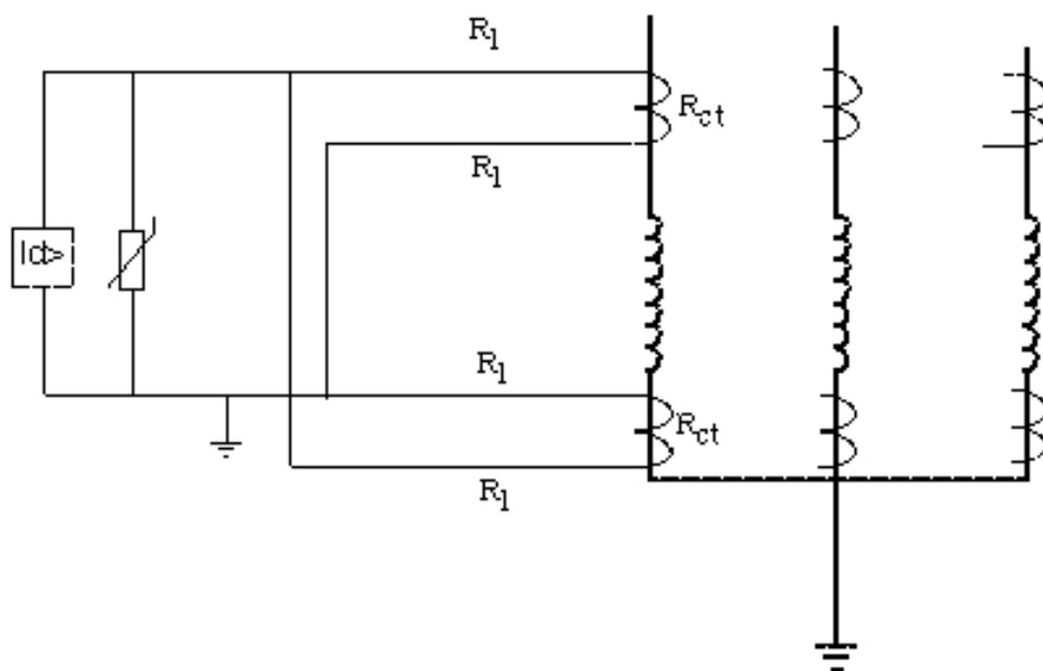
Figure 5. Connection principle for a high impedance differential protection.
