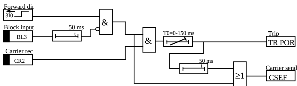
Figure 7. A permissive overreaching scheme (POR) with directional earth fault relays.
