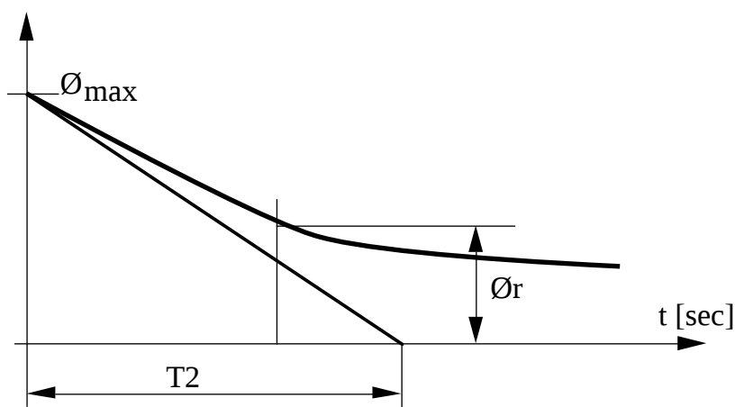
Figure 5. The decay of the flux and the remanence flux.
