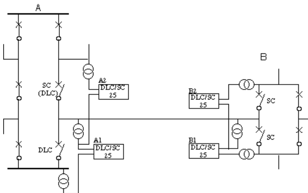
Figure 31. Dead line check and synchronism check at auto-reclosing in a One- and a half-breaker station and a Ring busbar station
