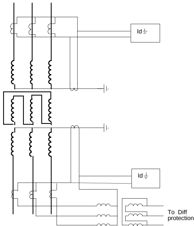
Figure 3. A restricted earth fault relay for an YNdyn transformer.
