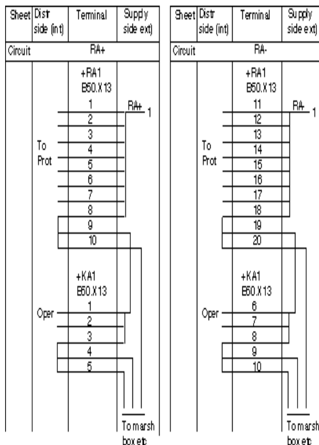
Figure 9. A terminal arrangement, enabling a simple localization of earth faults and a simple design of the DC distribution to different panels and boxes.
