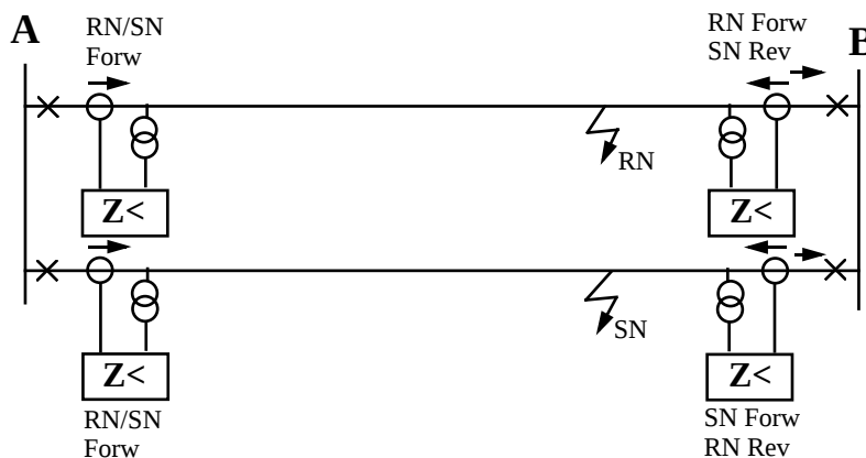
Figure 21. Simultaneous faults, in parallel lines, at the same tower.
