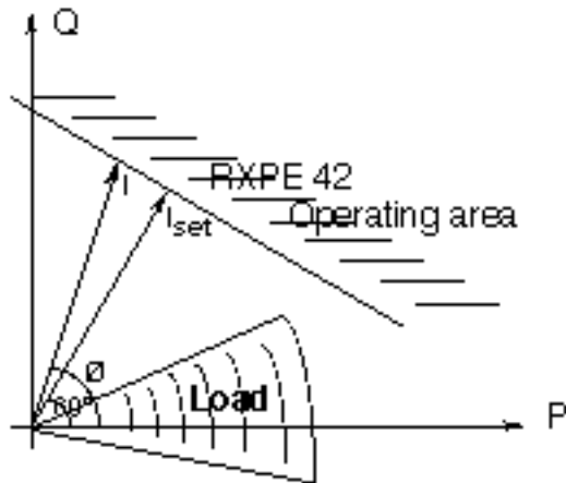
Figure 13. Directional short circuit protection, e. g. type RXPE 42 have 60-65° angle on characteristic for maximum sensitivity.
