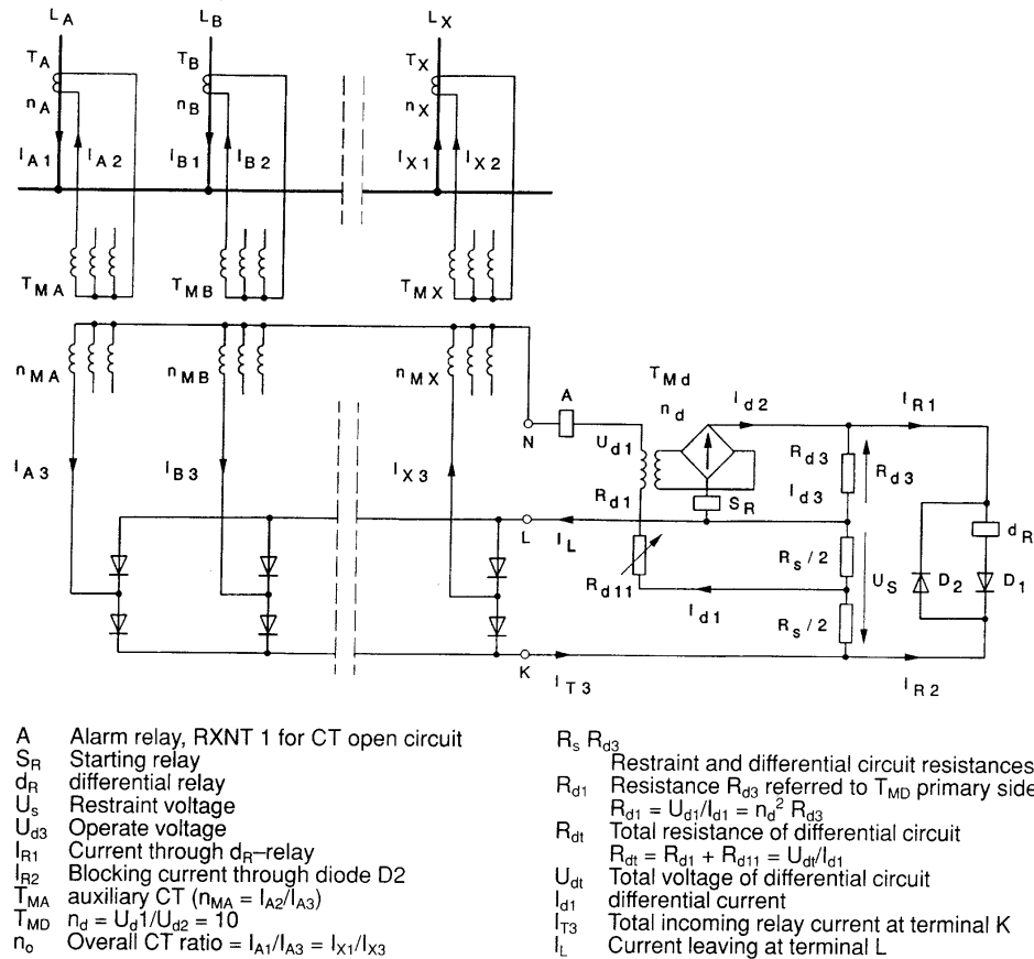
Figure 6. RADSS/REB 103 operating principle for one phase.
