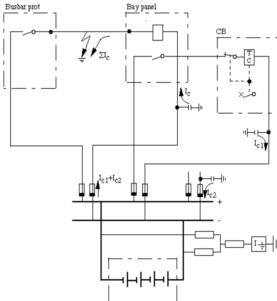
Figure 12. An earth fault in the battery system, will give capacitive discharges, which can operate trip relays. Secured trip relays should be used when the circuit is simply available e.g. in terminals.
