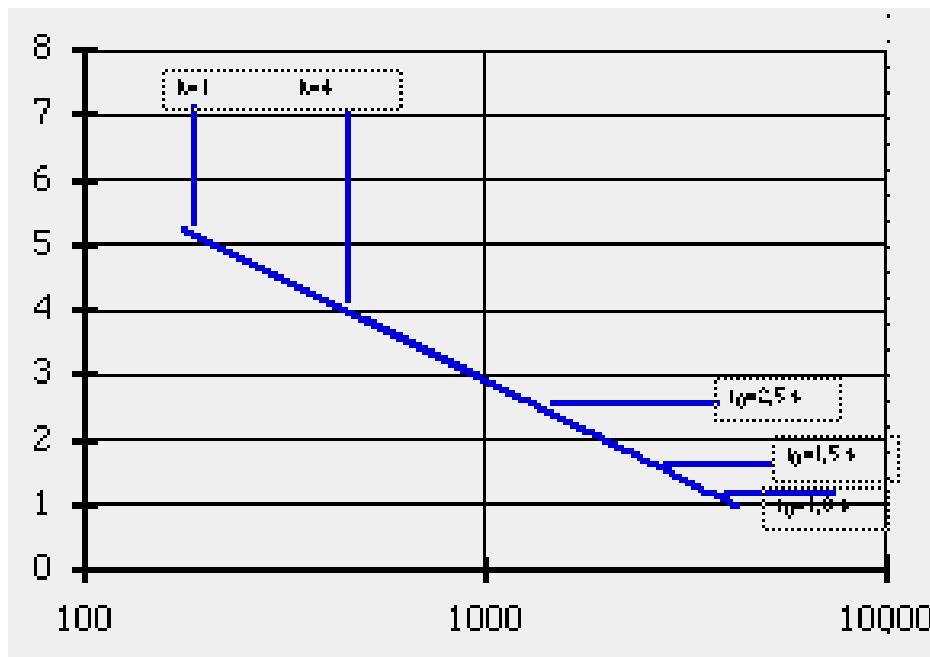
Figure 26. The logarithmic inverse characteristic will give selectivity if the biggest object fault current contribution is lower than 80% of the faulty object fault current.
