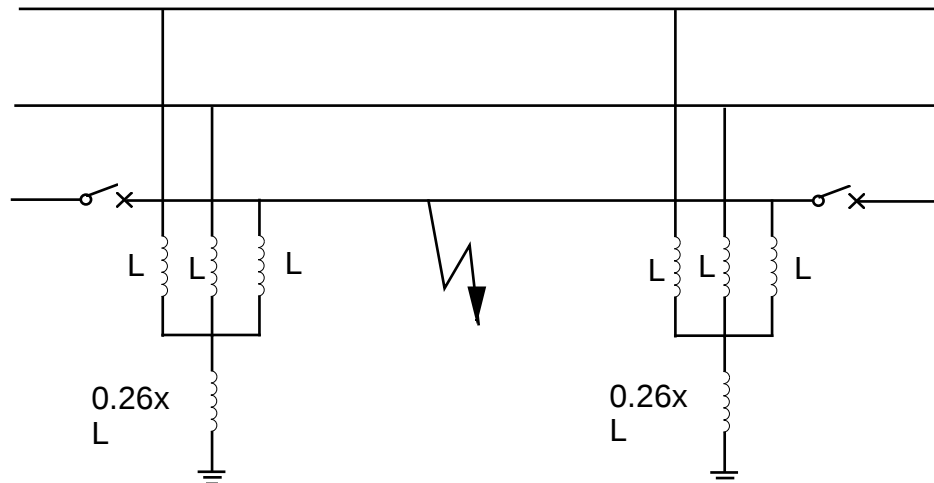
Figure 9. Single pole fault clearance on a power line with teaser reactors to extinguish the arc.
