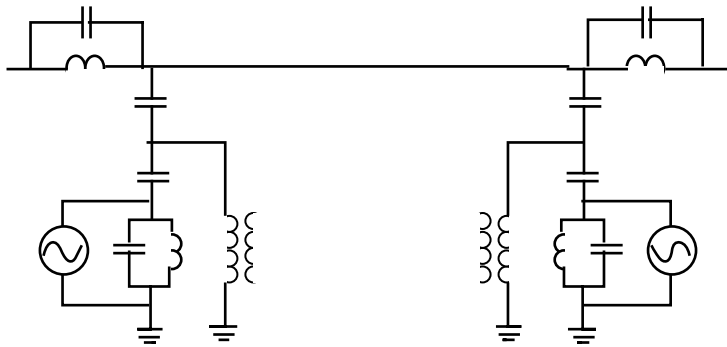
Figure 2. Communication through a high frequency signal, interposed at the high voltage line (PLC).
