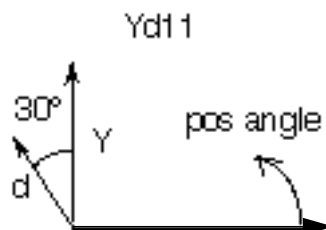
Figure 2. The positive sequence current is turned +30^\circ , while the negative sequence current is turned -30^\circ .
