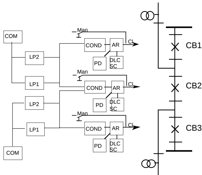
Figure 28. Auto-reclosers (AR) and cooperating equipment in a One- and a half-breaker bay
