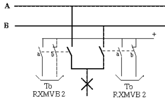
Figure 5. Requirements and connection of busbar disconnector auxiliary contacts, for switching of RXMVB 2 repeat relays.
