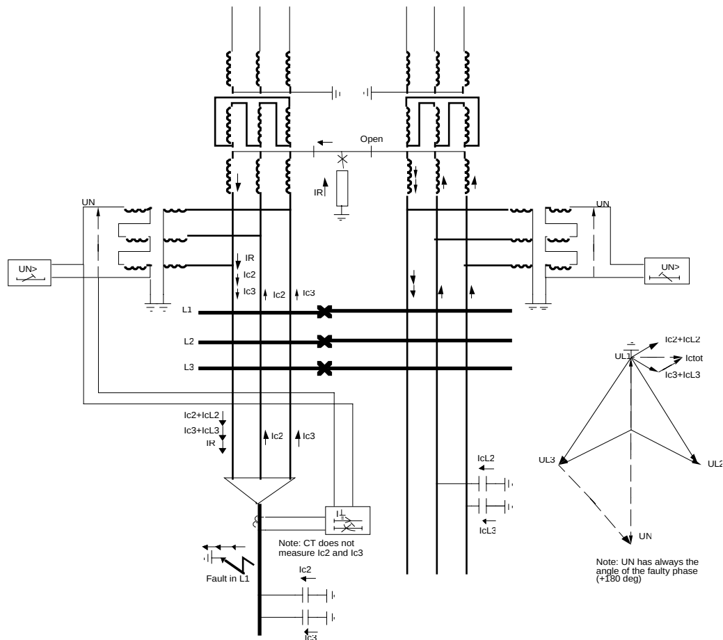
Figure 15. The fault and capacitive current distribution in a high resistance earthed network.
