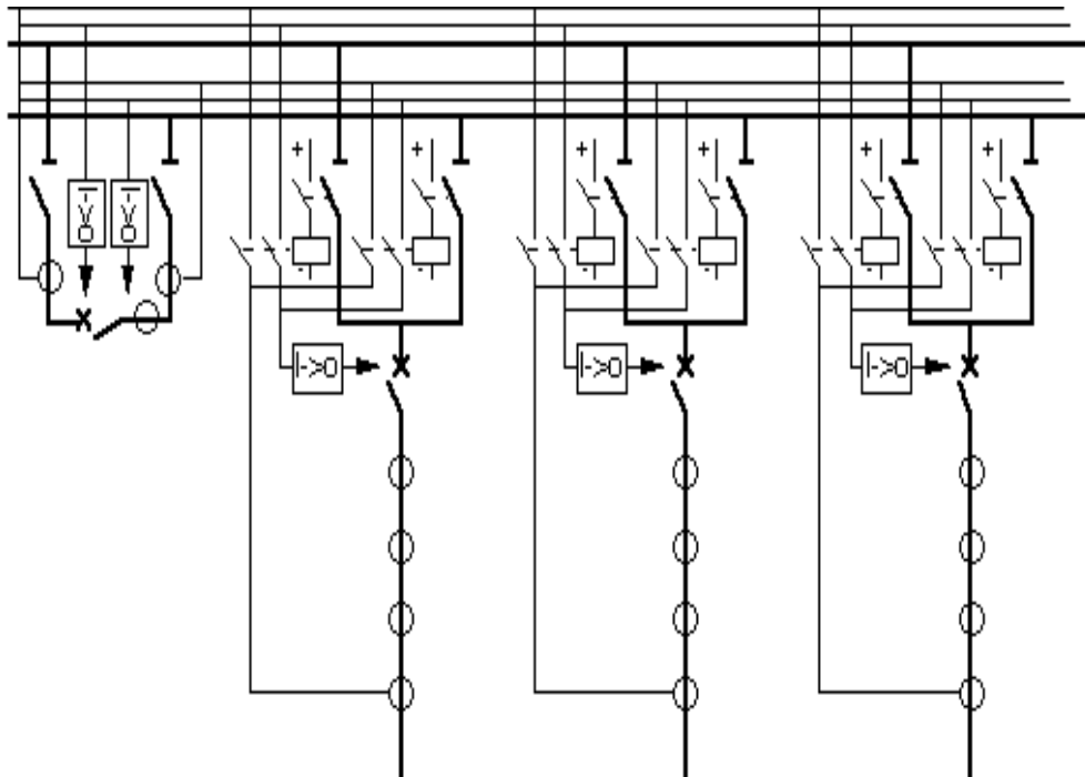
Figure 11. A trip busbar arrangement, for busbar protection tripping, gives a simple solution and allows the CBF trip to be connected without extra auxiliary circuits on the disconnectors.
