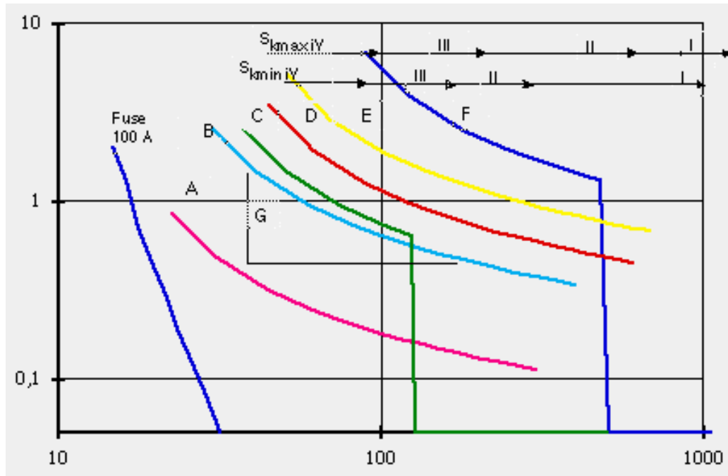
Figure 24. The selectivity plan will have all relays in the network indicated and the time margin must be checked for all selective relays. The sensitivity for back-up protection to fulfil tripping criteria must also be checked.
