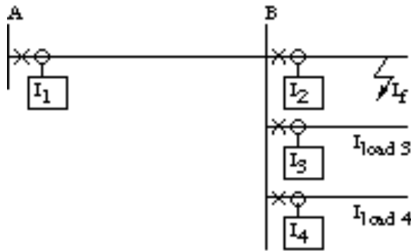
Figure 12. Setting of overcurrent relays must provide margin to maximum load current.
