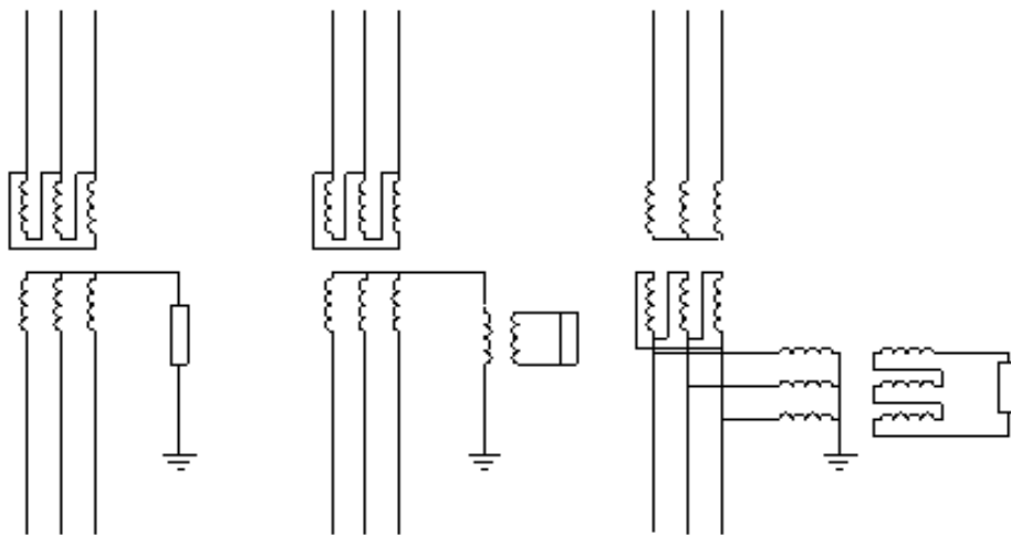
Figure 4. Three equal methods to prevent ferro resonance.
