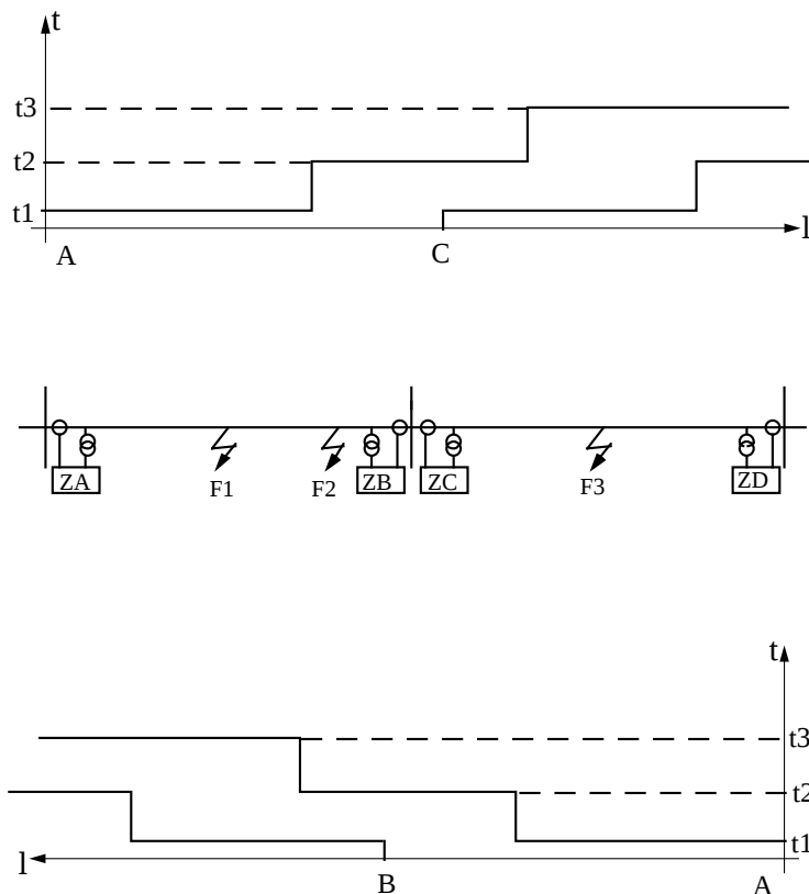
Figure 8. The principle of line protection, with Distance protection relays at both line ends.
