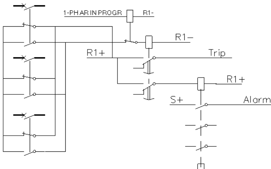
Figure 9. Connection of a Pole Discordance relay.
