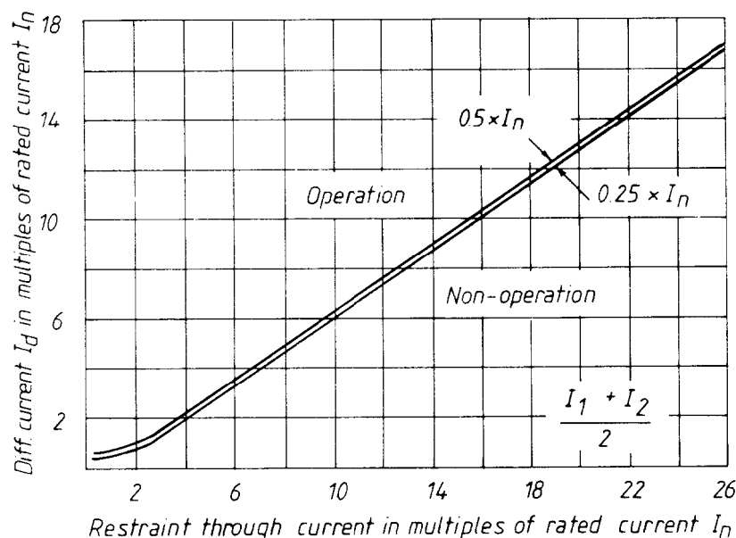
Figure 2. Through fault restraint gives an increased required differential current when the through fault current is increasing.
