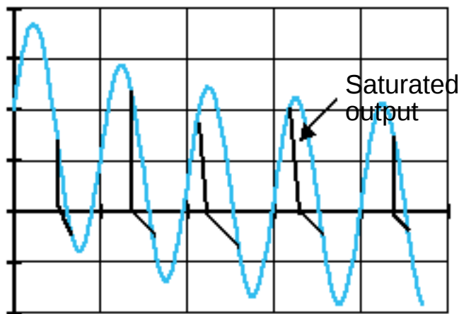
Figure 6. Secondary current at DC saturation. For some cycles the positive part of the sine wave will be destroyed.
