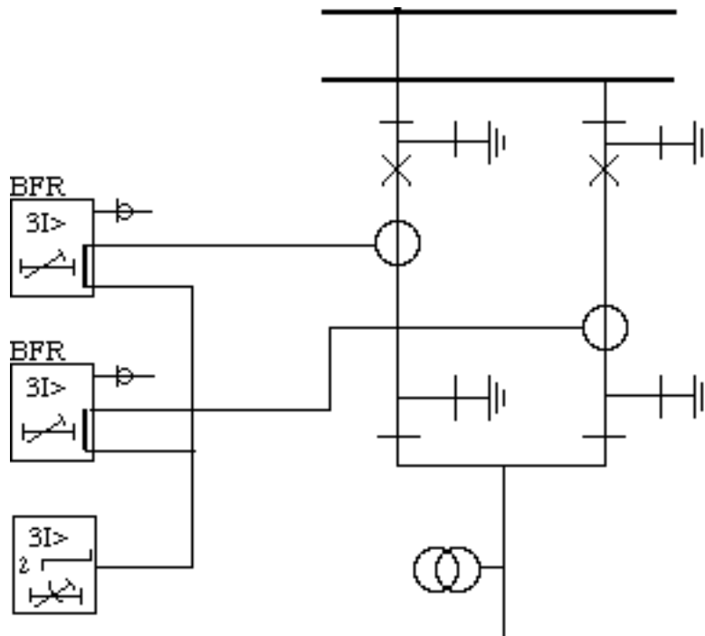
Figure 3. Summation of current transformers in a double busbar arrangement.
