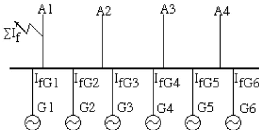
Figure 21. A generating station with many infeeds to a fault on an outgoing feeder.
