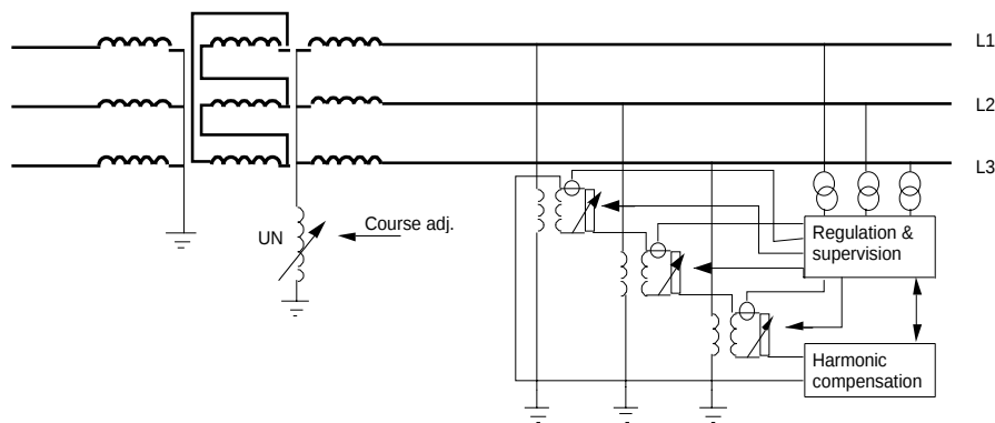
Figure 18. A compensation equipment for neutral point unsymmetry.
