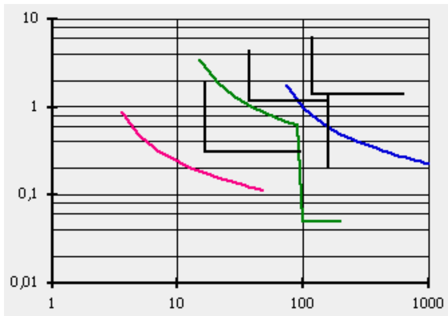
Figure 11. Inverse time delayed relays are at the same time current and time selective.
