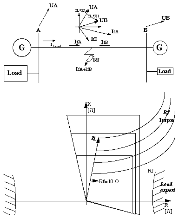
Figure 5. The Distance protection export end will overreach when a fault resistance is added in a double end infeed system. The import end will underreach.
