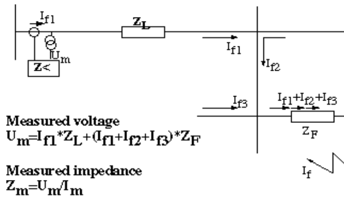
Figure 4. A fault at a remote station will due to infeed from other objects be seen as much further off than it really is.
