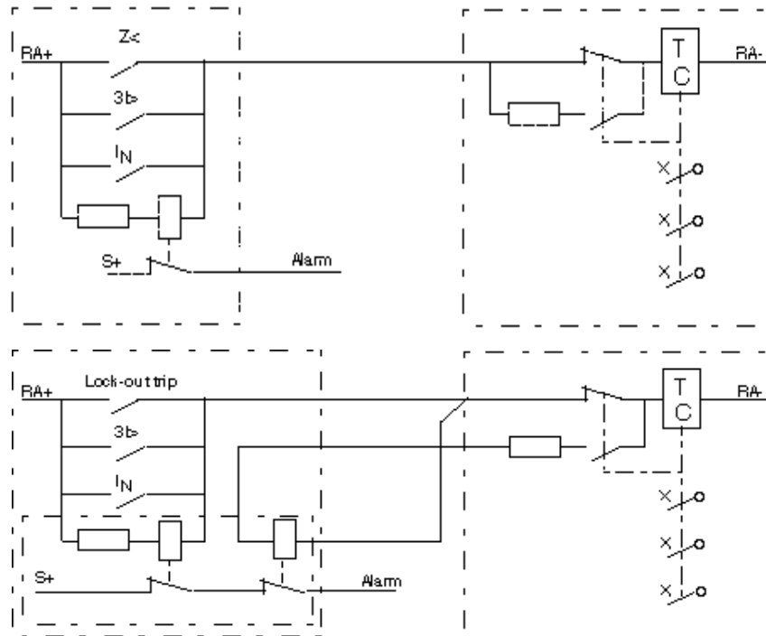
Figure 10. Arrangement of a trip circuit supervision. a) Single supervision, b) Double supervision (with lock-out trip relays).
