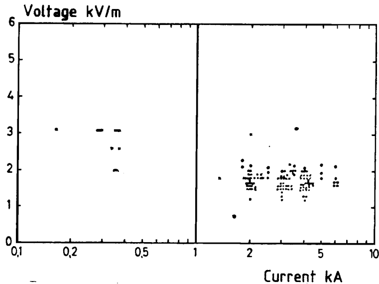
Figure 3. Distribution of arc voltage and current at many tests in ASEA.
