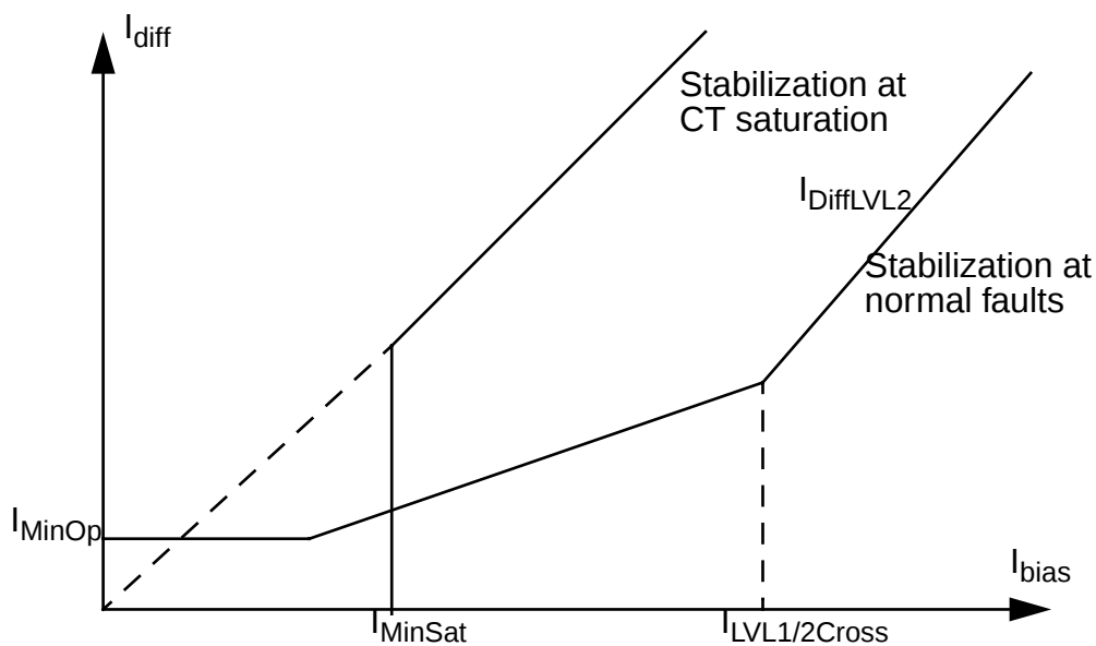
Figure 5. The stabilization characteristic.
