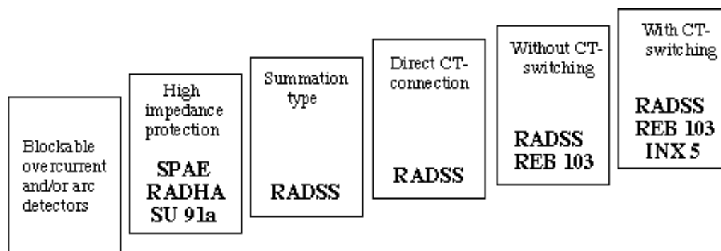
Figure 7. Application of different types of busbar protection relays
