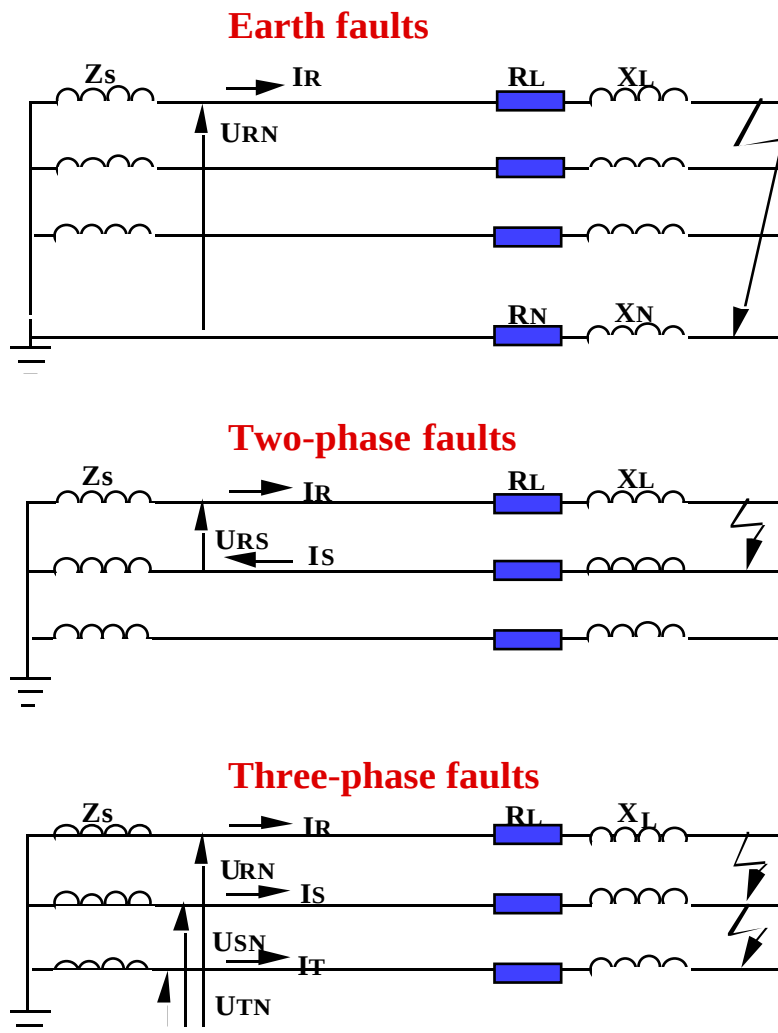
Figure 10. The impedance measuring loops for different fault types.
