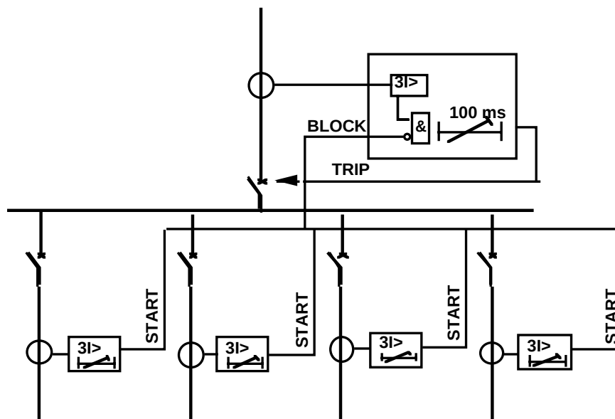
Figure 6. Blockable Overcurrent protection.
