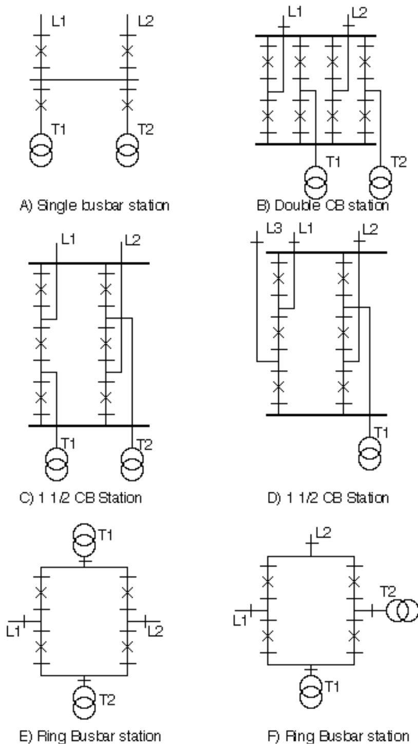
Figure 25. Examples of multi breaker switchgear arrangements
