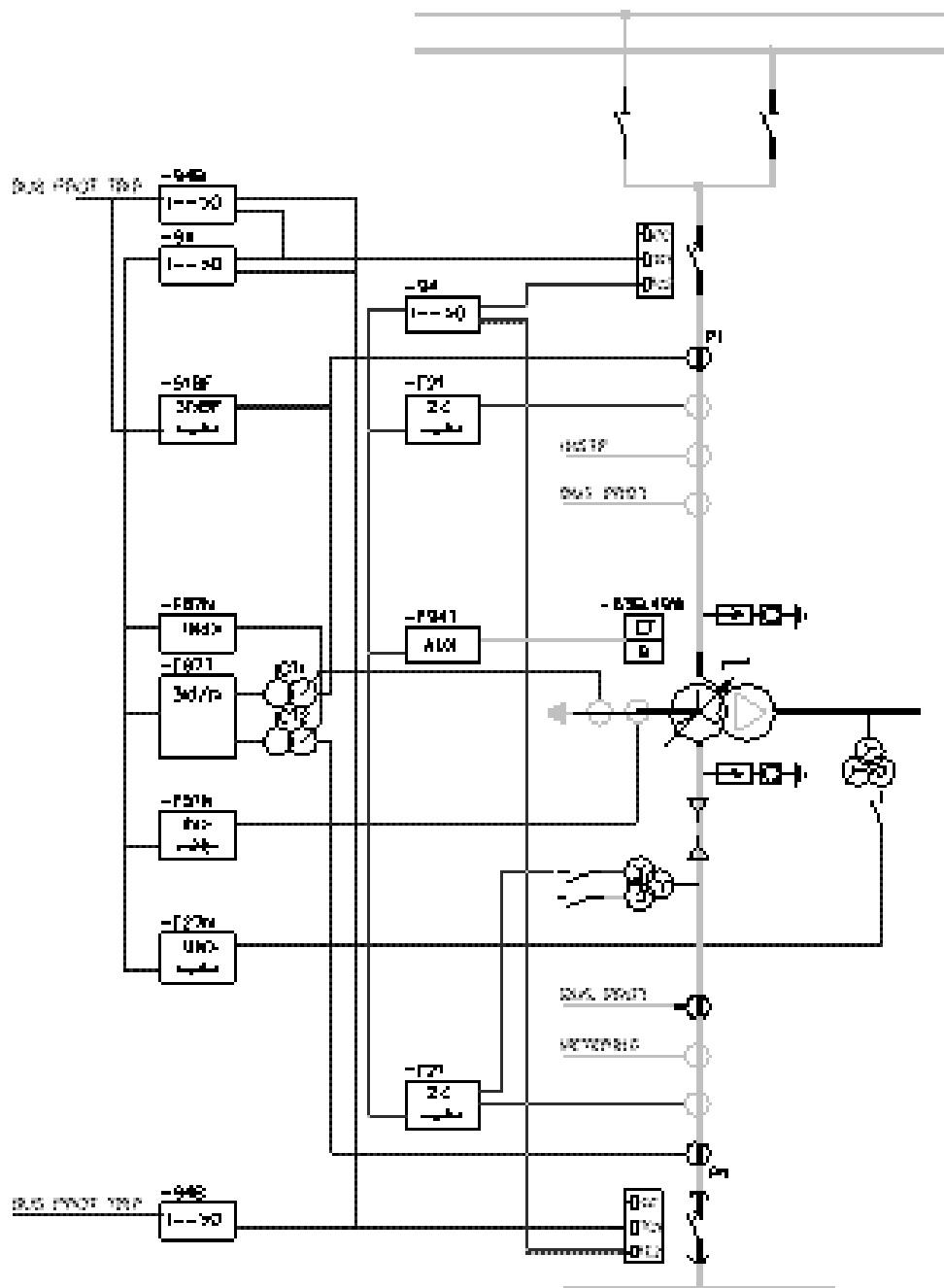
Figure 6. A typical protection system for a EHV/HV system power transformer.
