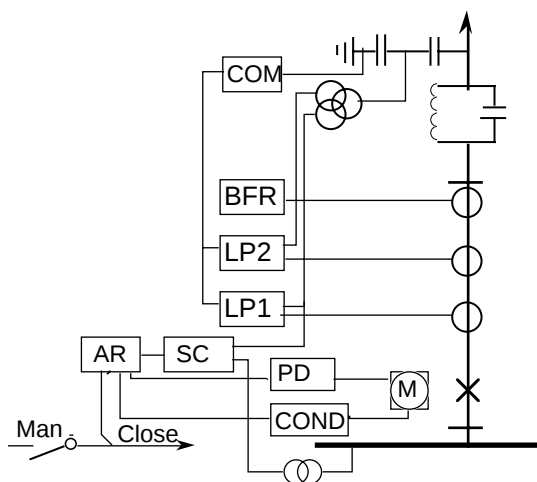
Figure 22. The Auto recloser and communicating equipment in a line bay.
