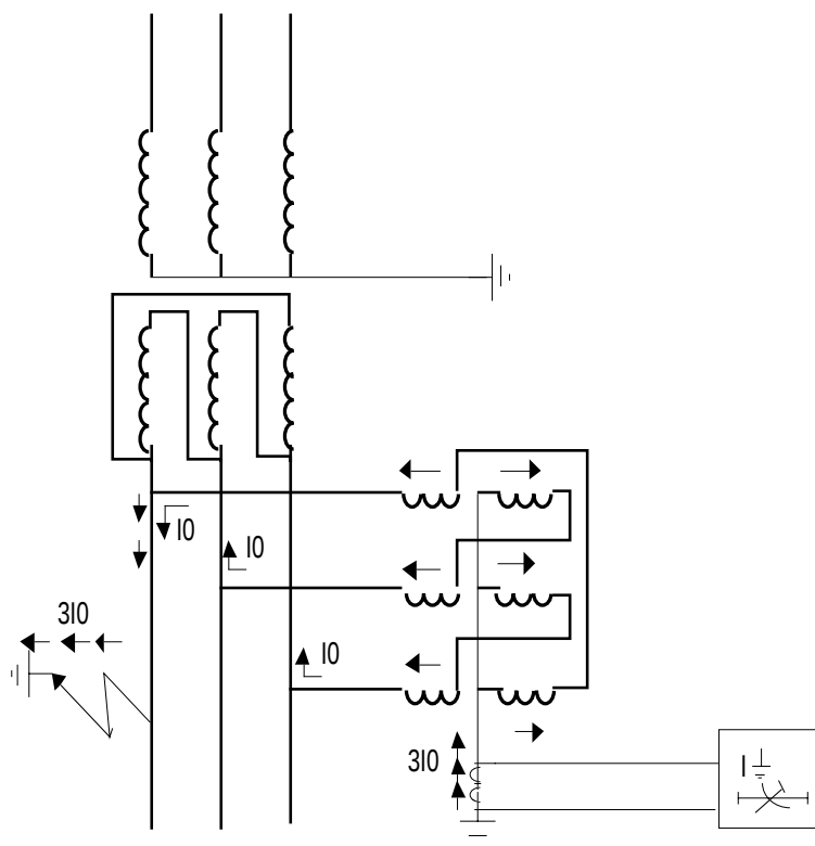
Figure 13. An earth fault protection system for a reactance earthed network where selectivity is achieved by inverse time delayed relays.
