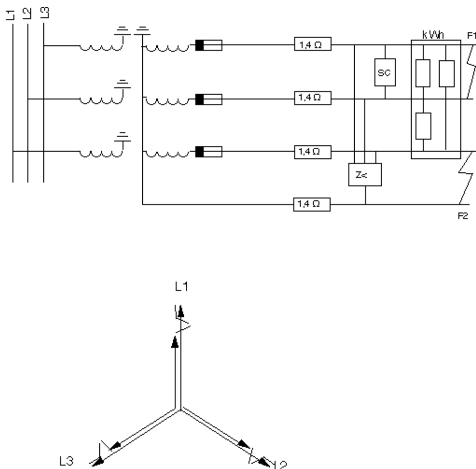
Figure 8. The voltage drop for a voltage transformer secondary circuit.
