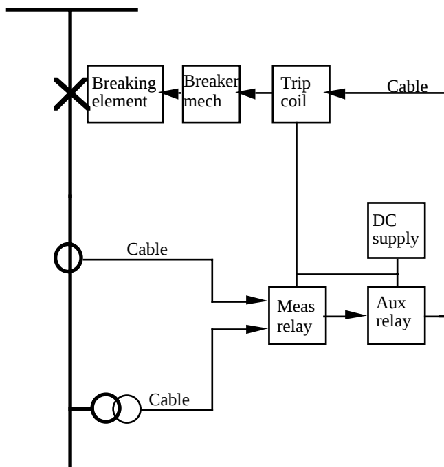
Figure 1. The different parts of the fault clearance chain
