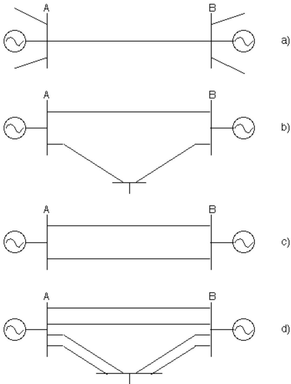
Figure 29. Power grid with different degree of meshing between A and B
