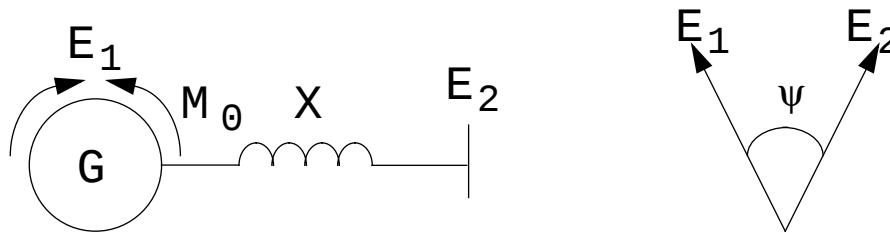
Figure 5. Generator feeding a “strong” network.
