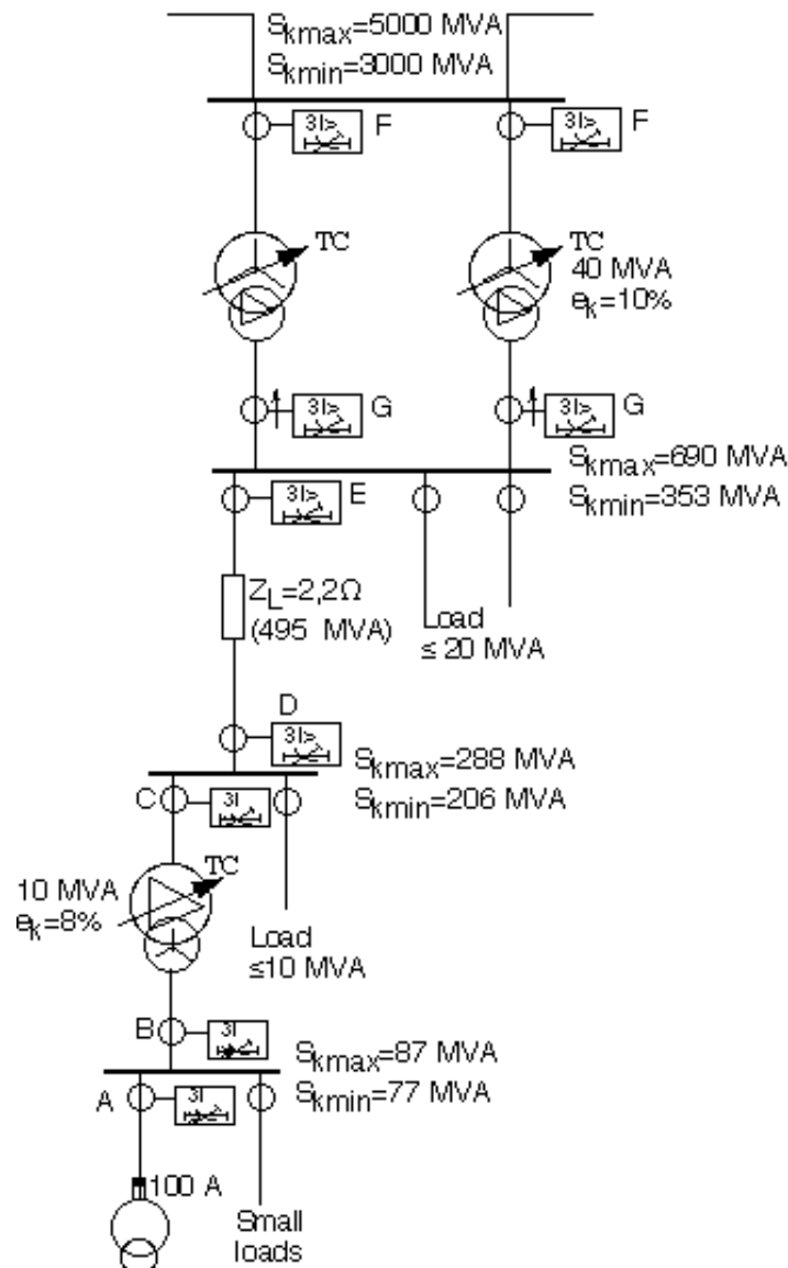
Figure 23. The selectivity plan must cover setting of all the protection relays in the network.
