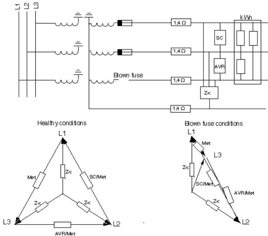
Figure 7. Back-feed of voltages to a faulty phase, when phase to phase load exists.
