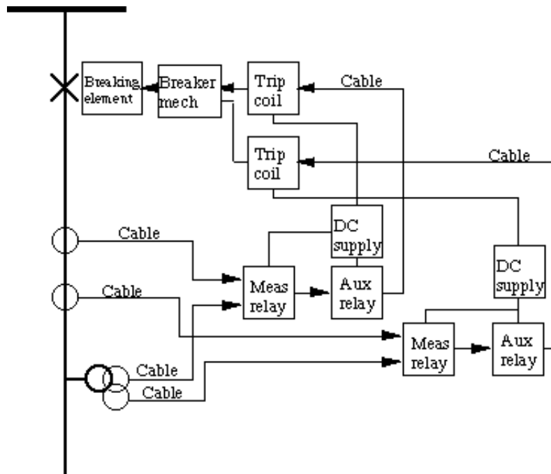
Figure 2. Fault clearance chain at redundant protection systems
