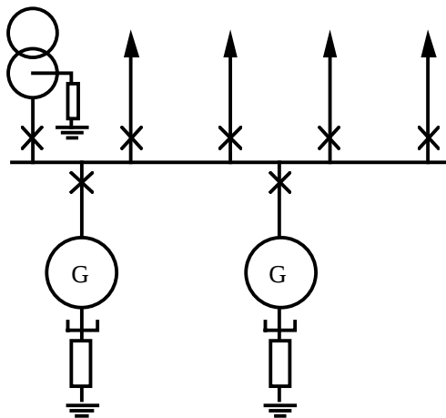
Figure 10. Earthing individual neutral-point with impedances.
