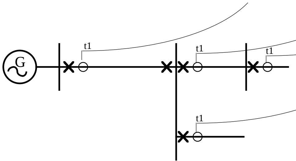
Figure 5. Back-up protection with time grading.
