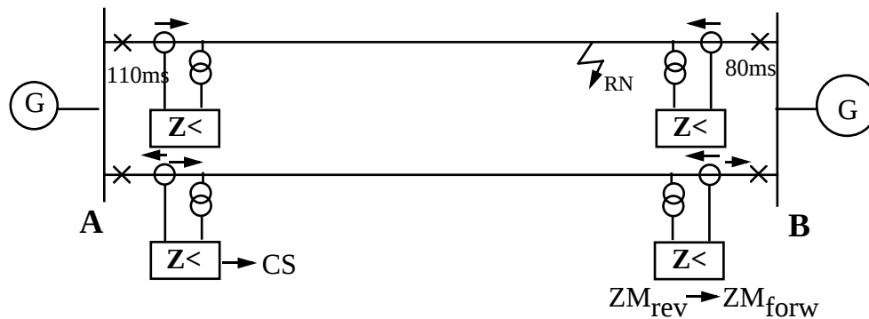
Figure 19. Fault current reversal occurring, with parallel lines, at the same tower.
