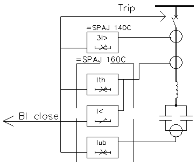
Figure 2. A SPAJ 160 connected to a capacitor bank.
