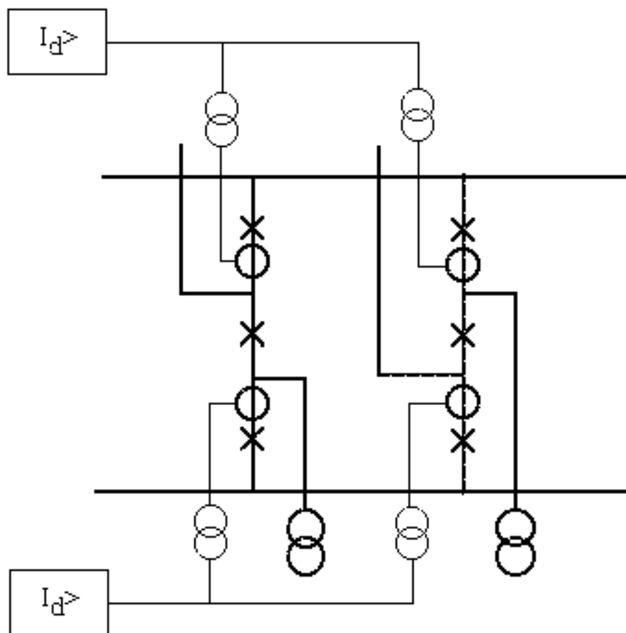
Figure 2. A two-zone busbar differential relay for 1 1/2-breaker switchgear
