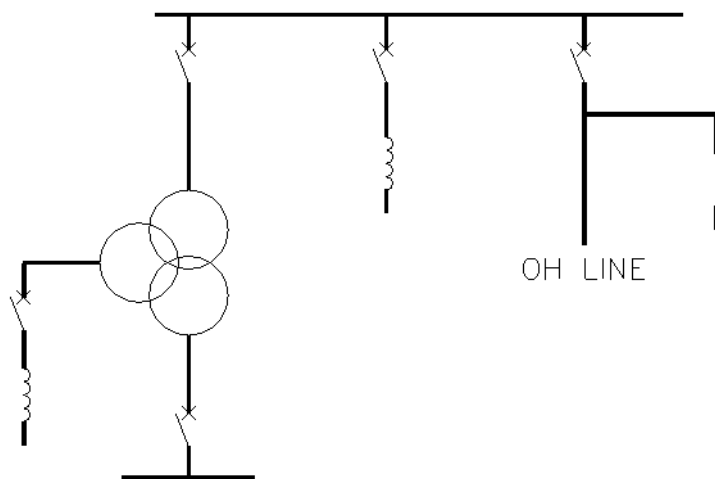
Figure 1. Different locations of shunt reactors.
