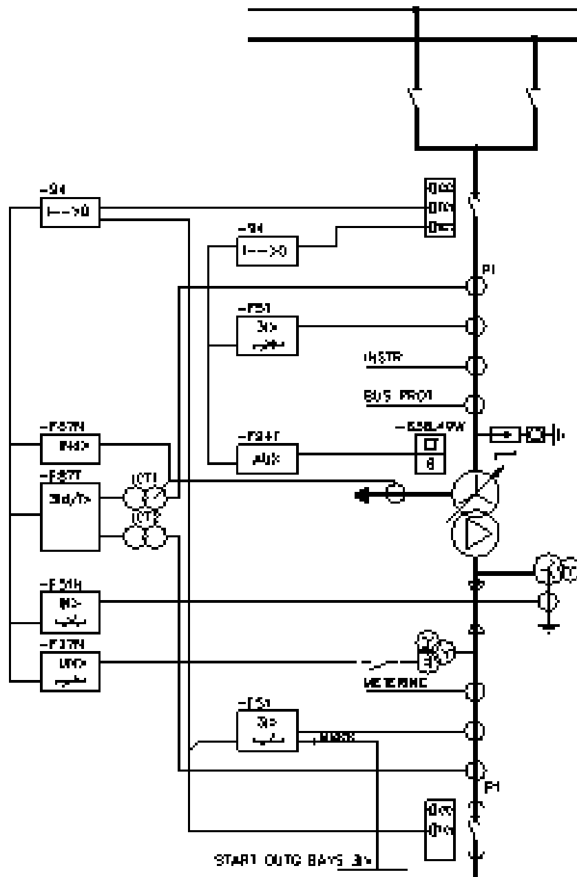
Figure 5. A typical protection system for a HV/MV power transformer.
