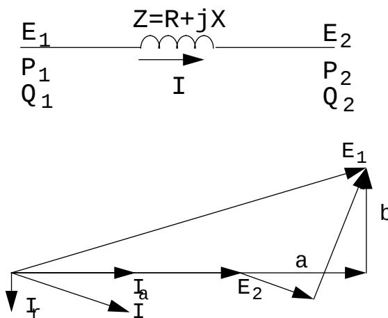
Figure 3. Load transfer on a short line.
