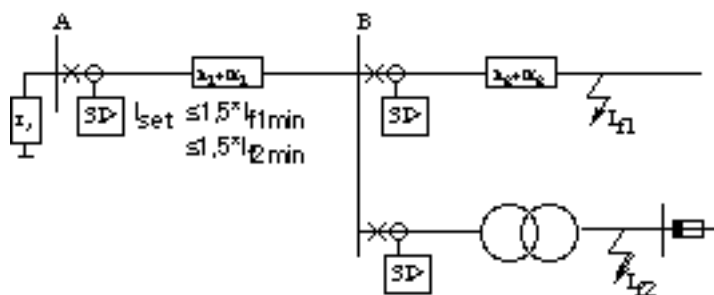
Figure 15. The minimum fault current achieved for which the overcurrent relay is required to be back-up must be detected.
