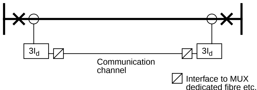
Figure 4. The principle for an optical line differential relay with one protection relay at each line end communicating through a communication channel.
