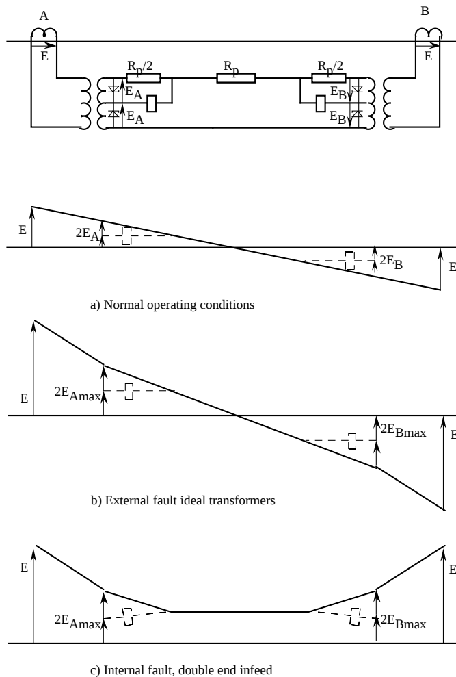
Figure 3. A voltage balance current differential relay
