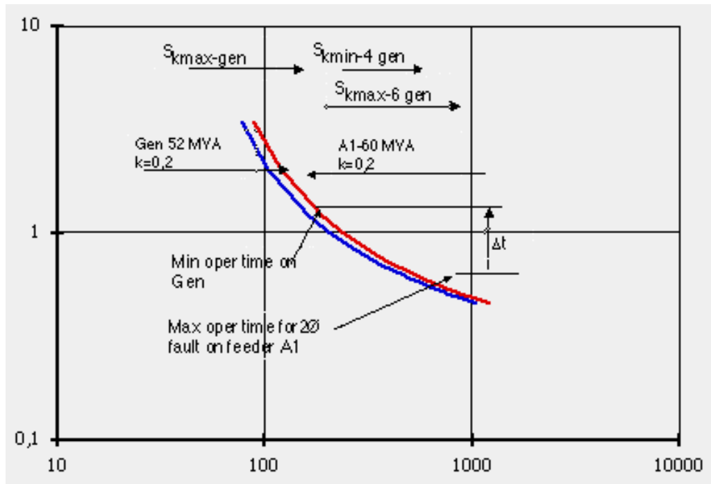
Figure 22. Similar settings can give selectivity due to differences in fault currents at different locations.
