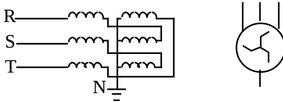
Figure 6. Z/0-connected earthing transformer.
