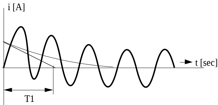
Figure 4. The primary fault current with a DC component.
