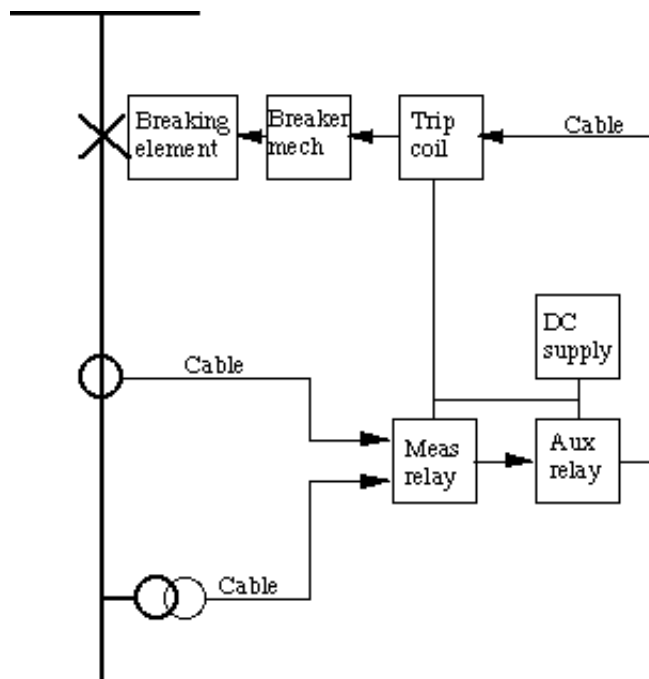
Figure 3. The different parts of the fault clearance chain.
