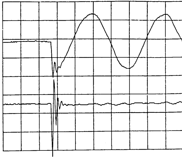
Figure 19. The neutral point voltages and the high frequency transient occurring at an earth fault.
