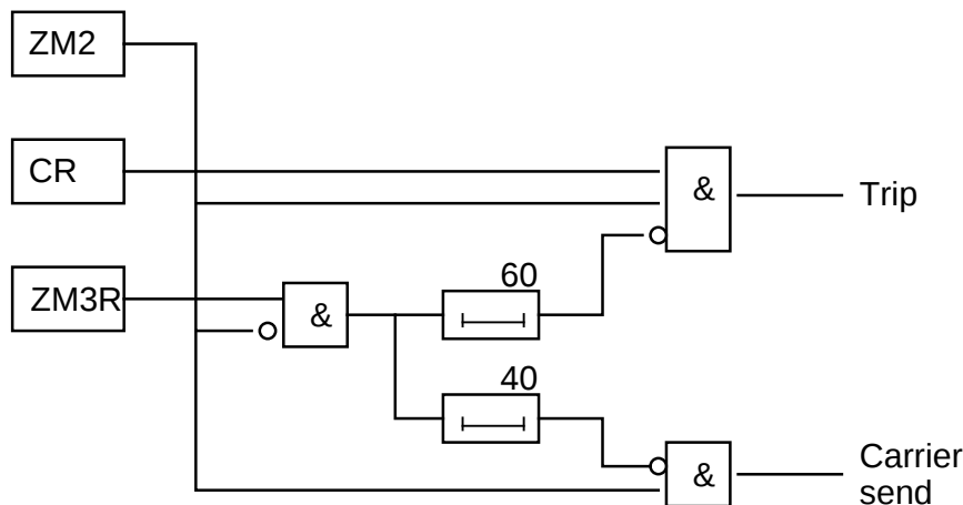
Figure 20. Fault current reversal logic for overreaching scheme in RELZ 100/REL 511/521./531 “ZM2” is measuring zone 2, “ZM3R” is Zone 3 reverse and “CR” is carrier receive.
