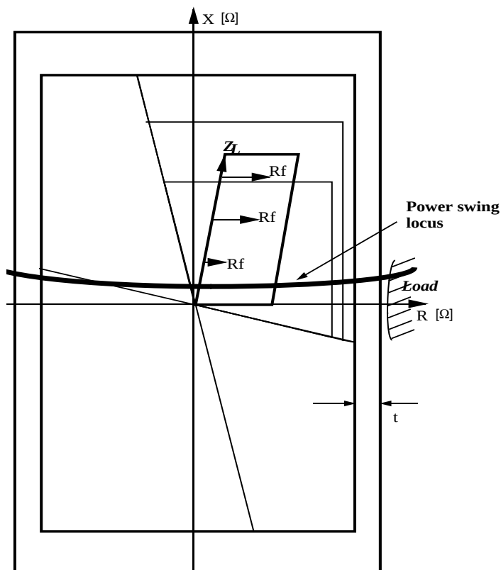
Figure 17. Power Swing Blocking function. Two rectangles can be provided and the time between passing the outer and inner rectangle is measured.
