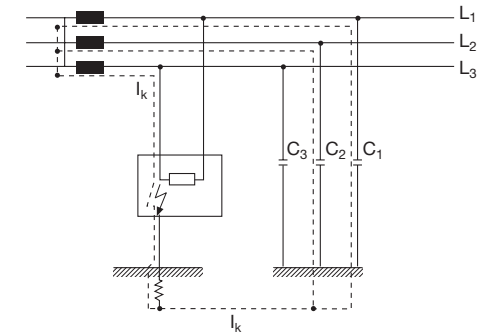
Figure 3: Earth fault in IT systems
