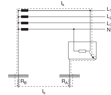
Figure 1: Earth fault in TT system
