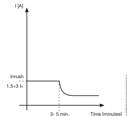
Inrush current diagram
