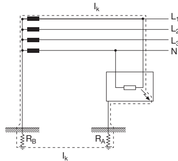
Figure 1: Earth fault in IT systems
