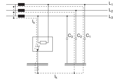
Figure1: Earth fault in IT system
